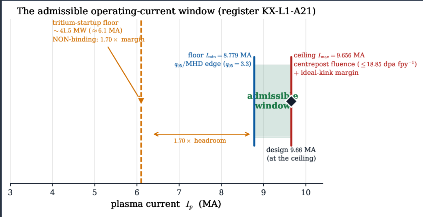
The admissible operating-current window (KX-L1-A21). Floor I_{\min} = 8.779 MA set by the q_{95} /MHD edge; ceiling I_{\max} = 9.656 MA co-set by centrepost fluence and ideal-kink margin. The design current 9.66 MA sits at the ceiling. The tritium-startup floor ( \approx 6.1 MA) is non-binding, with 1.70\times headroom.
