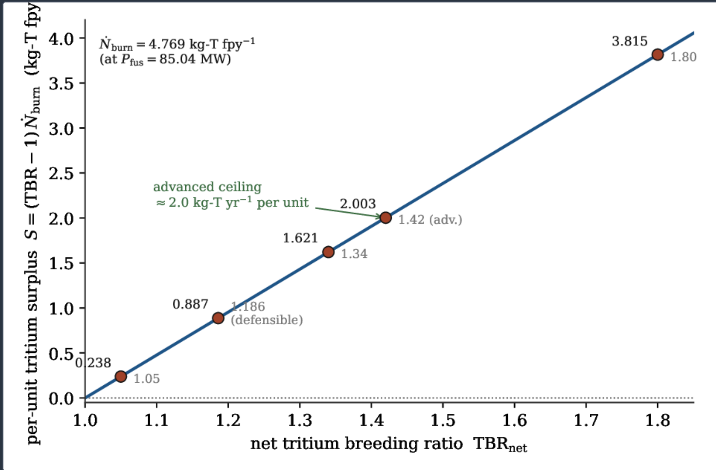
Per-unit tritium surplus S = (\text{TBR} - 1)\dot{N}_{\text{burn}} at \dot{N}_{\text{burn}} = 4.769\text{kg} - T\backslash\text{ensuremath fpy}^{-1} . Markers are register anchors; the advanced ceiling yields \approx 2.0\text{kg-T yr}^{-1} per unit. The plant is a consumer where S < 0 and an exporter where S > 0 .
