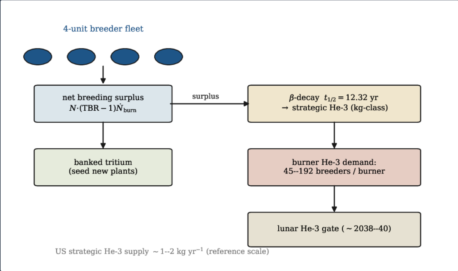
(Schematic.) The tritium-to-helium-3 flywheel of a four-unit breeder fleet. Net breeding surplus is banked, seeds new plants, and \beta -decays ( t_{1/2} = 12.32 \text{ yr} ) into strategic helium-3; burner-scale helium-3 demand ( 45–192 breeders per burner) stays lunar-gated.
