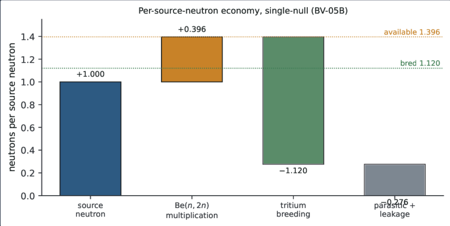
Per-source-neutron economy in single-null (BV-05B), a graphical form of the balance equation (7). One source neutron plus 0.396 beryllium (n, 2n) neutrons give 1.396 available; of these 1.120 are consumed in tritium breeding and 0.276 go to parasitic absorption and leakage.
