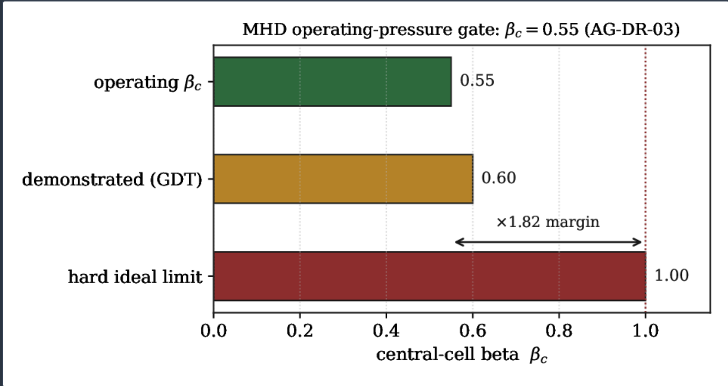
MHD operating-pressure gate. The central-cell \beta_c = 0.55 sits a factor 1.82 below the hard \beta = 1 ideal limit and next to the demonstrated gas-dynamic-trap value ( \sim 0.6 ). Data: AG-DR-03.
