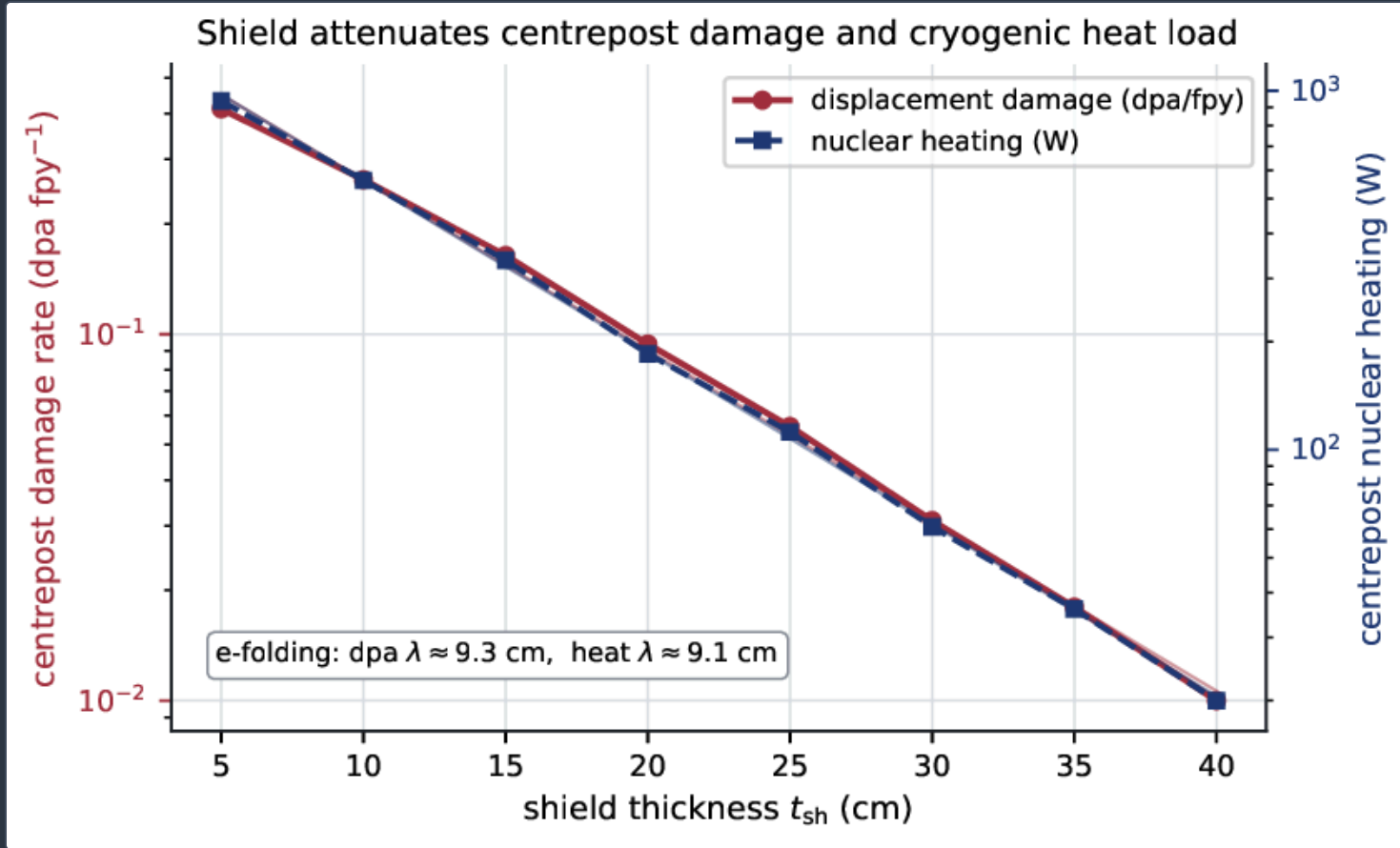
Shield attenuation of centrepost displacement damage (red, dpa/fpy) and nuclear heating (navy, W) versus t_{sh} ; both axes are logarithmic and the faint lines are single-exponential fits with the quoted e-folding lengths. The heat curve is the coupling into the cryogenic budget (gates BR-L1-A13b, BR-L1-A13).
