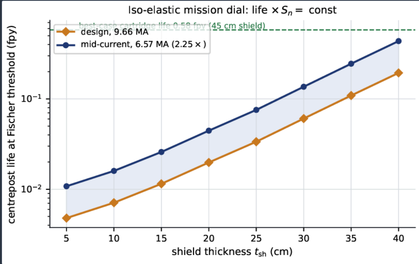
Iso-elastic mission dial (equation 5): centrepost life at the Fischer threshold for the design ( 9.66 MA ) and mid-current ( 6.57 MA ) points, separated everywhere by the exact factor 2.25 . The dashed line marks the best-case 0.58 fpy cartridge life at the fully shielded ( 45 cm ) end.
