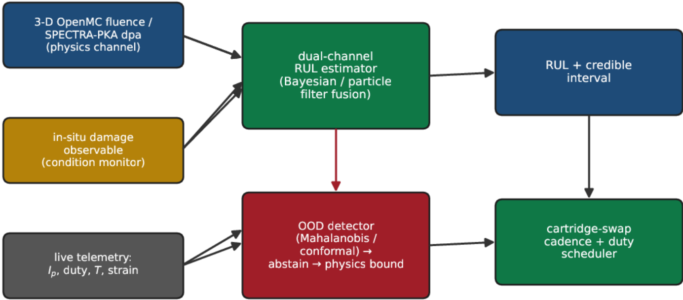
Prognostic architecture: two channels, one backstop, a scheduled decision
