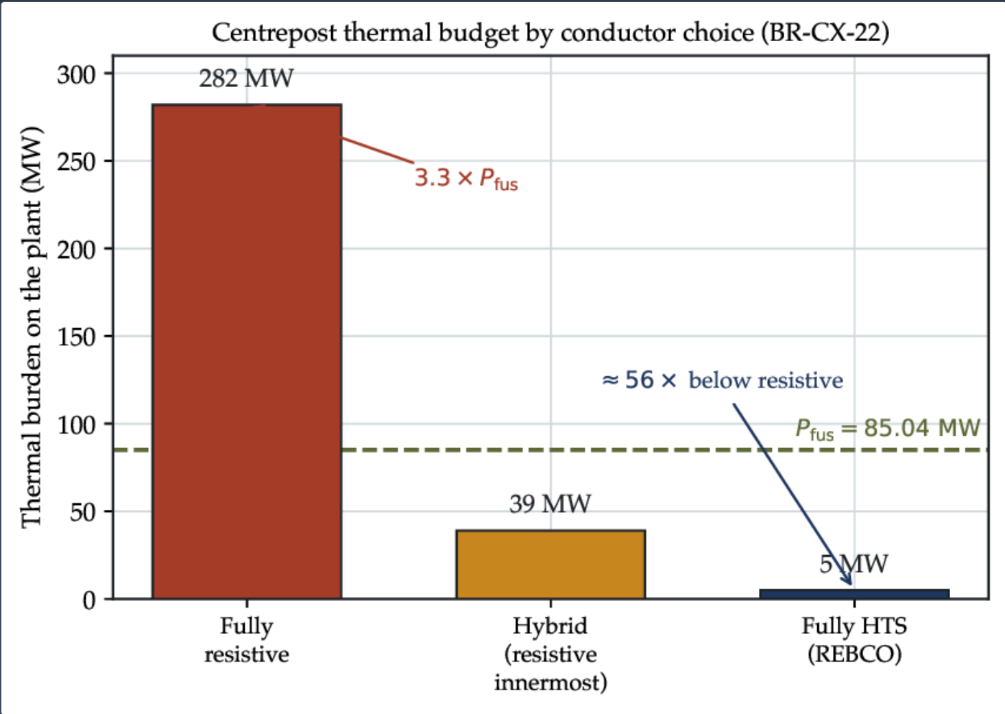
Centrepost thermal budget by conductor choice (BR-CX-22). A fully-resistive post dissipates \approx 282\text{ MW} ( 3.3 \times P_{fus} ); a hybrid keeps only a \approx 39\text{ MW} resistive sacrificial innermost layer; a fully superconducting post reduces the burden to an \approx 5\text{ MW} cryogenic load, \approx 56\times below resistive. The dashed line marks P_{fus} = 85.04\text{ MW} .
