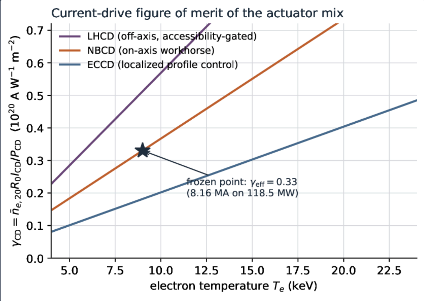
Current-drive figure of merit \gamma_{CD} = \bar{n}_{e,20} R_0 I_{CD} / P_{CD} versus T_e for the three mechanisms (equation (13); mechanism constants representative). The star marks the frozen aggregate \gamma_{\text{eff}} = 0.33 implied by 8.16 MA on 118.5 MW .
