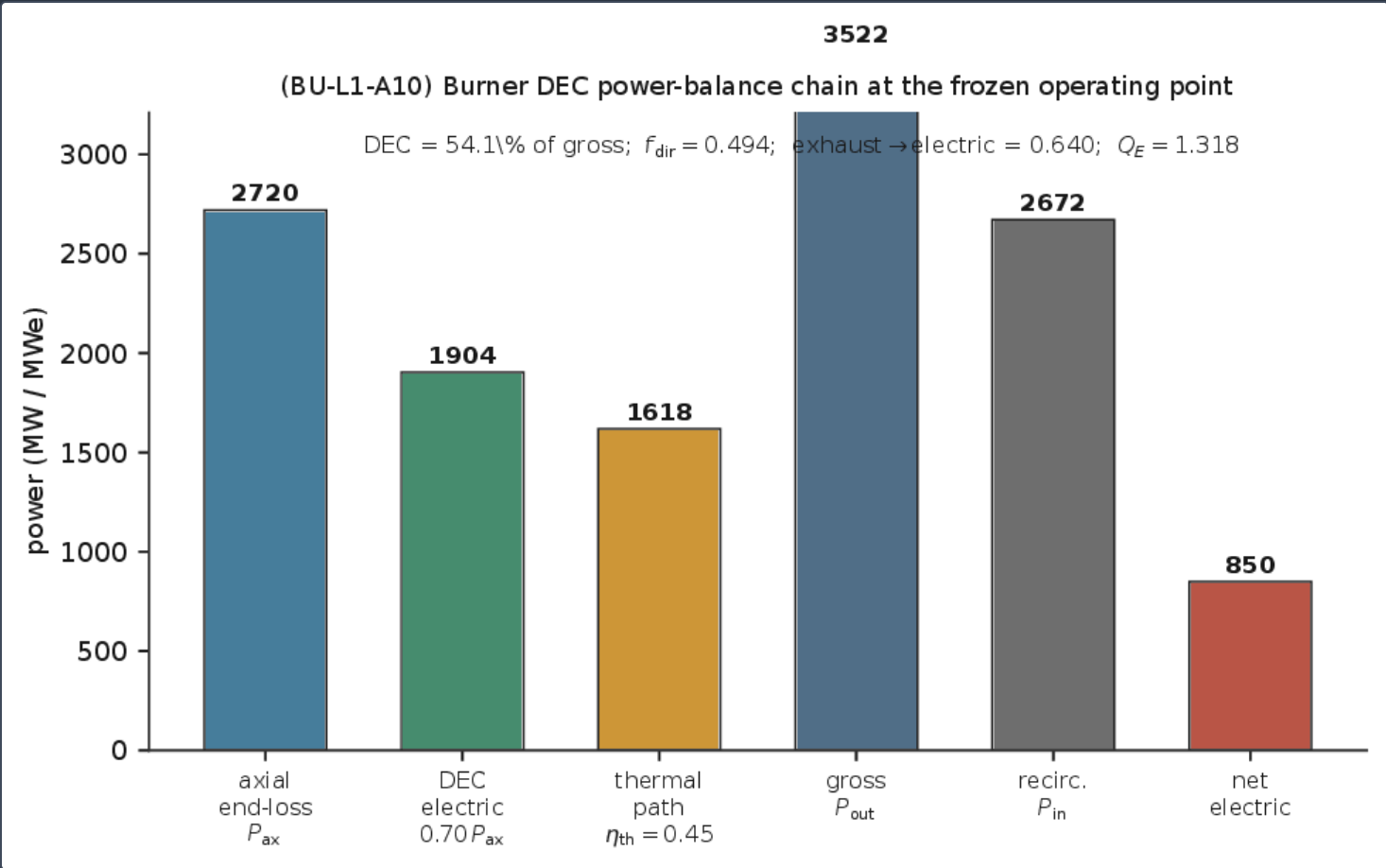
Burner DEC power-balance chain at the frozen operating point (BU-L1-A10), Eq. 10. Axial end-loss P_{\text{ax}} = 2719.7 MW; DEC electric 1903.8 MWe ( 54.1% of gross); thermal recovery 1618.2 MWe; gross 3522.0 MWe; recirculating 2672.0 MWe; net 850 MWe; Q_E = 1.318 , exhaust-to-electric 0.640 .
