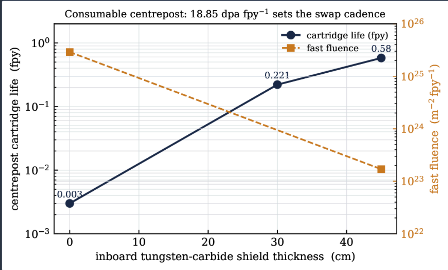
Consumable-centrepost life versus inboard tungsten-carbide shield thickness (left axis) and the corresponding fast-fluence rate (right axis). Anchored at register points BR-L1-A13b (0, 45 cm) and SC-BR-2 (30 cm); the connecting curve is a monotone interpolation of the anchors.
