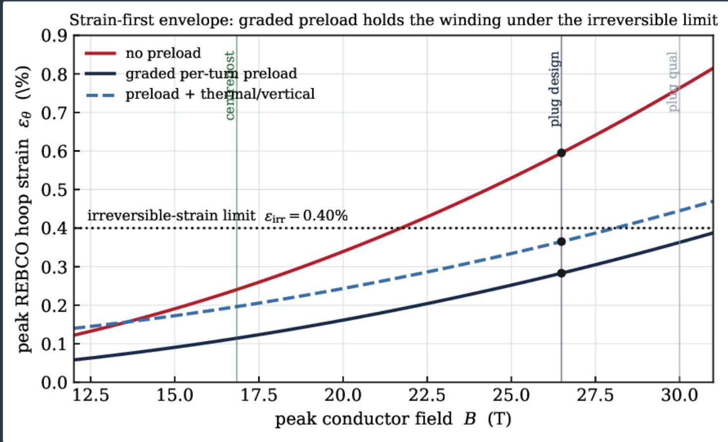
Strain-first envelope: peak REBCO hoop strain versus field for no pre-load, graded per-turn pre-load, and pre-load with thermal/vertical loads superposed, against the 0.40% irreversible limit. Curves are derived from the frozen finite-element anchors (register SC-BR-4, HX-09; markers) through the p_{mag} \propto B^2 Lorentz scaling, with the thermal/vertical contribution modelled as a field-independent offset.
