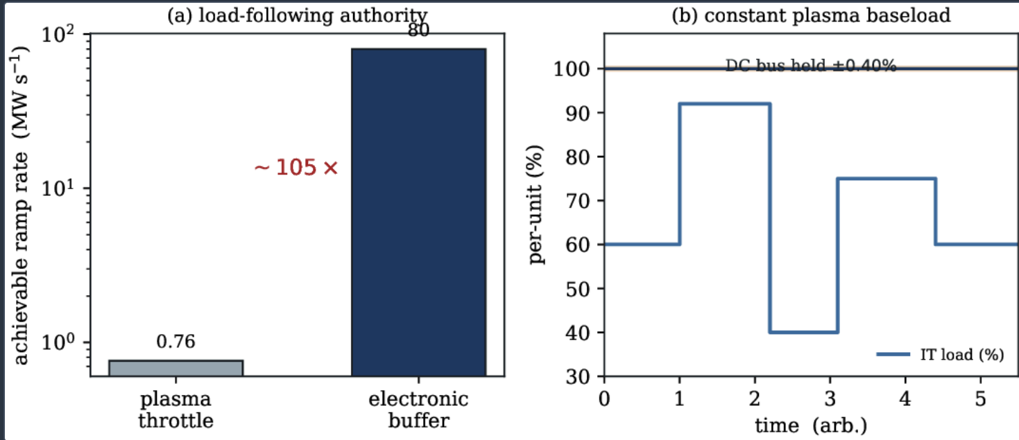
Electronic load-following at constant plasma baseload (BU-CX-07, BU-CX-08). (a) The electronic buffer follows load at \sim 80\text{ MW s}^{-1} , about 105\times the plasma throttle authority. (b) Across 60 \rightarrow 92 \rightarrow 40 \rightarrow 75\% IT-load steps the closed-loop controller holds the DC bus within \pm 0.40\% while the plasma runs at a constant baseload; the trace is illustrative, the band and load steps are the frozen result.
