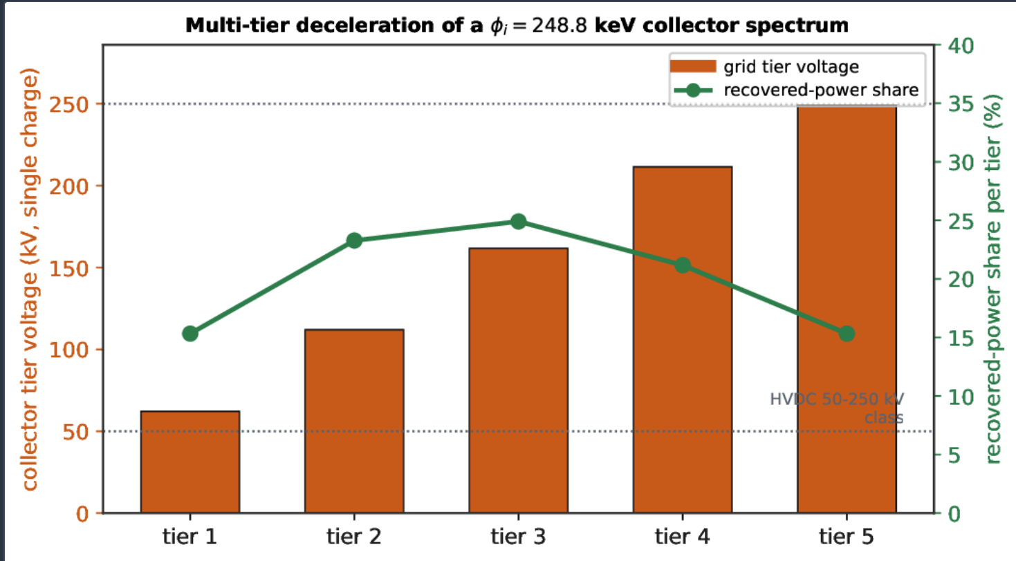
Multi-tier deceleration of a \phi_i = 248.75\text{ keV} collector spectrum (equation 2). Grid-tier voltages fall in the HVDC class; the recovered-power share is largest in the middle tiers. Tier weights are illustrative of a spectrum-matched collector.
