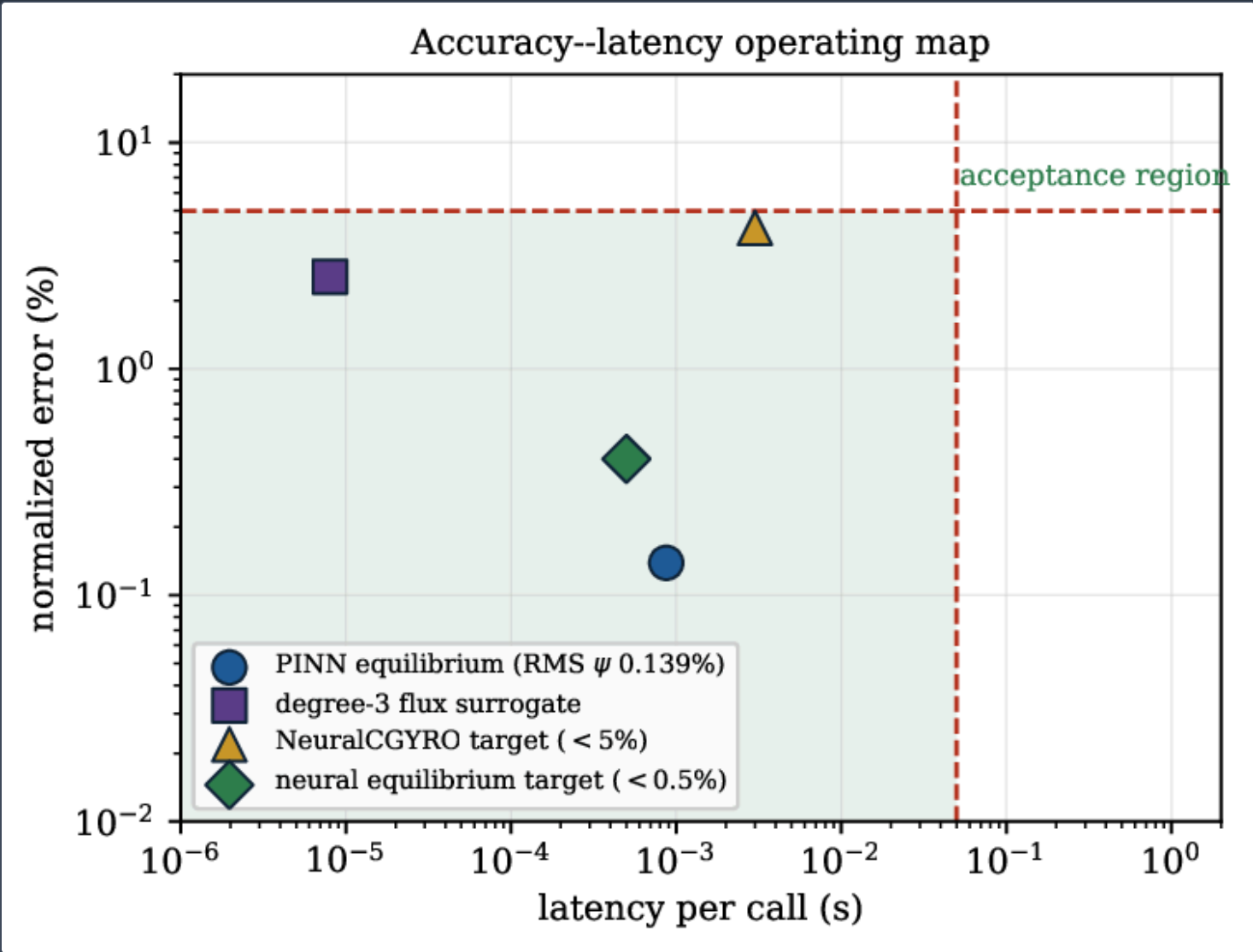
Accuracy–latency operating map. The shaded region is the acceptance envelope (latency \leq 50\text{ ms} , normalised error \leq 5\% ). Demonstrated operators (degree-3 flux surrogate; PINN equilibrium at 0.139% ) sit deep inside; the neural flux and neural equilibrium targets are placed at their pre-registered bounds. Both axes logarithmic.
