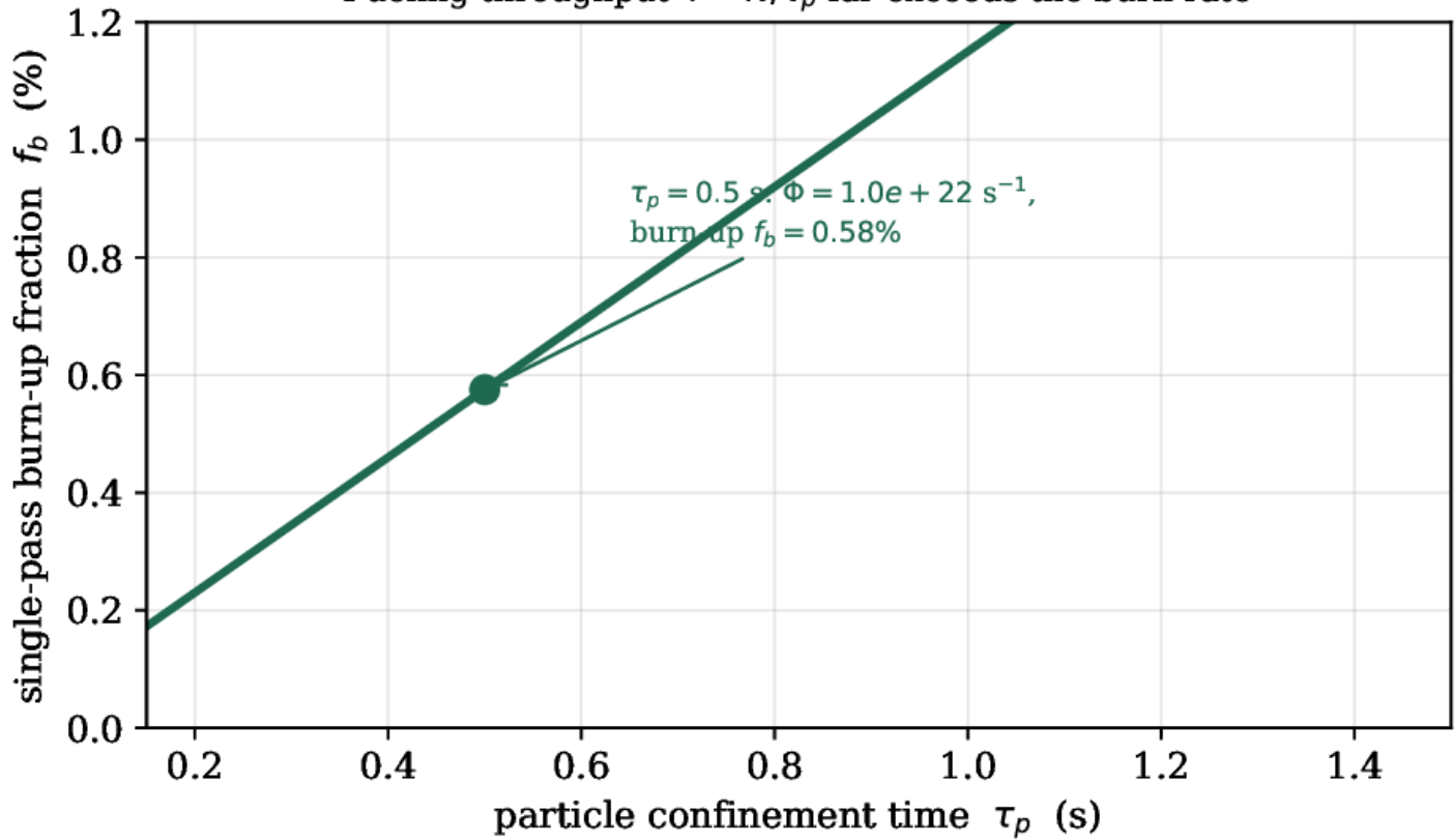
Fueling throughput \Phi = N/\tau_p far exceeds the burn rate
