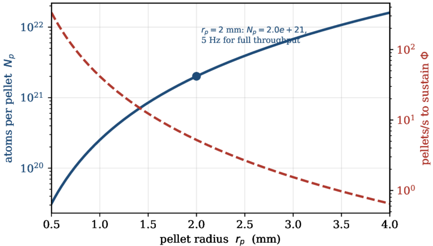
Pellet mass budget and injection cadence
