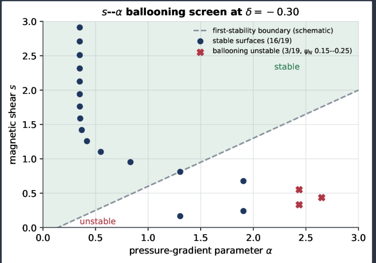
s -- \alpha ballooning screen. Sixteen of nineteen surfaces sit in the stable region; three low-shear core surfaces ( \psi_N \approx 0.15 – 0.25 ) cross the first-stability boundary. The boundary curve is schematic; the surface loci are the equilibrium values. (Schematic boundary.)
