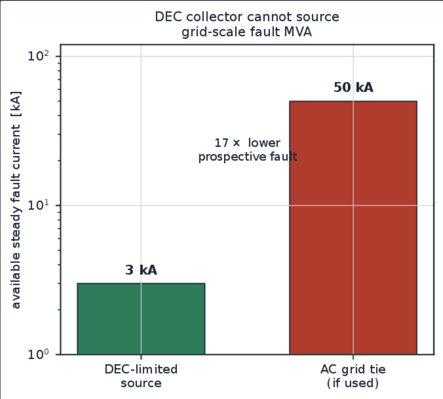
Decision (iii), source fault (MV-CX-05). Available steady fault current (log scale): the DEC collector is current-limited to ~3 kA , against ~50 kA from an AC grid tie— 17× lower prospective fault current, hence lower arc-flash energy and easier protection.
