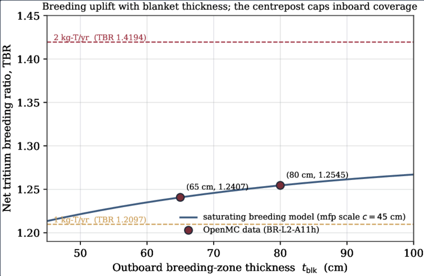
Net TBR versus outboard breeding-zone thickness (gate BR-L2-A11h). Markers are OpenMC data at 65 and 80 cm; the curve is a saturating breeding model (neutron-mean-free-path scale c = 45\text{ cm} ) through the two points. Horizontal lines are the 1\text{ kg} - T_{\text{ensured}}\text{yr}^{-1} and 2\text{ kg} - T_{\text{ensured}}\text{yr}^{-1} surplus bars. The centrepost caps inboard coverage, so the per-unit ceiling saturates at net TBR 1.42 .
