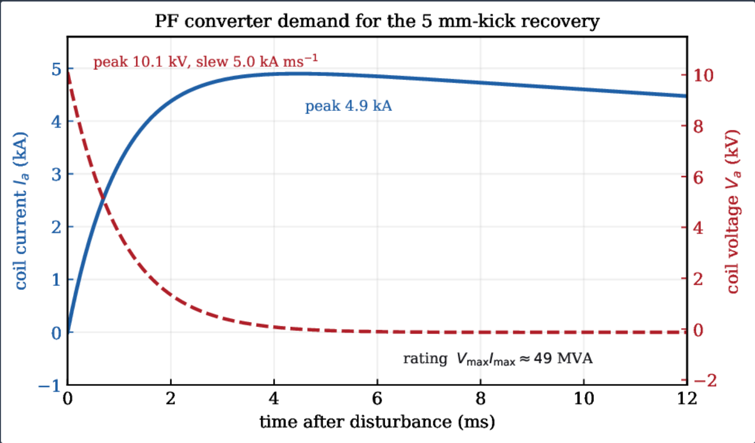
PF-converter demand during the 5 mm-kick recovery: coil current (left axis) peaks at 4.9 kA and drive voltage (right axis) at 10.1 kV, at a slew of 5.0 kA/ms, for a rating of \sim 49 Mvoltampere (equation 17).
