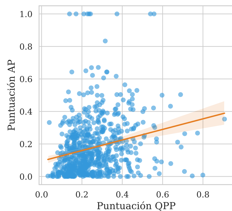
UEF-NQC \tau = 0.1981
