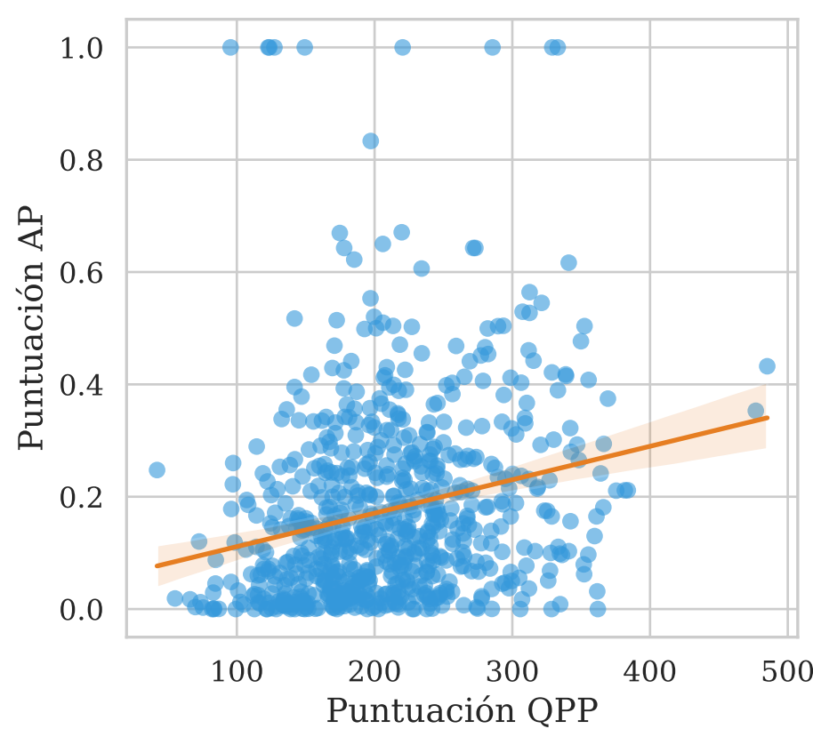
UEF-Clarity \tau = 0.1929
