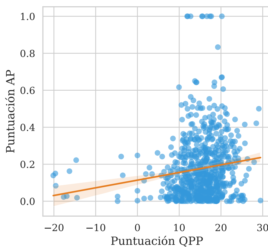
UEF-WIG \tau = 0.1143
