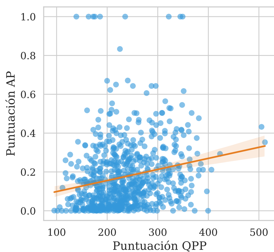
Clarity \tau = 0.1747
