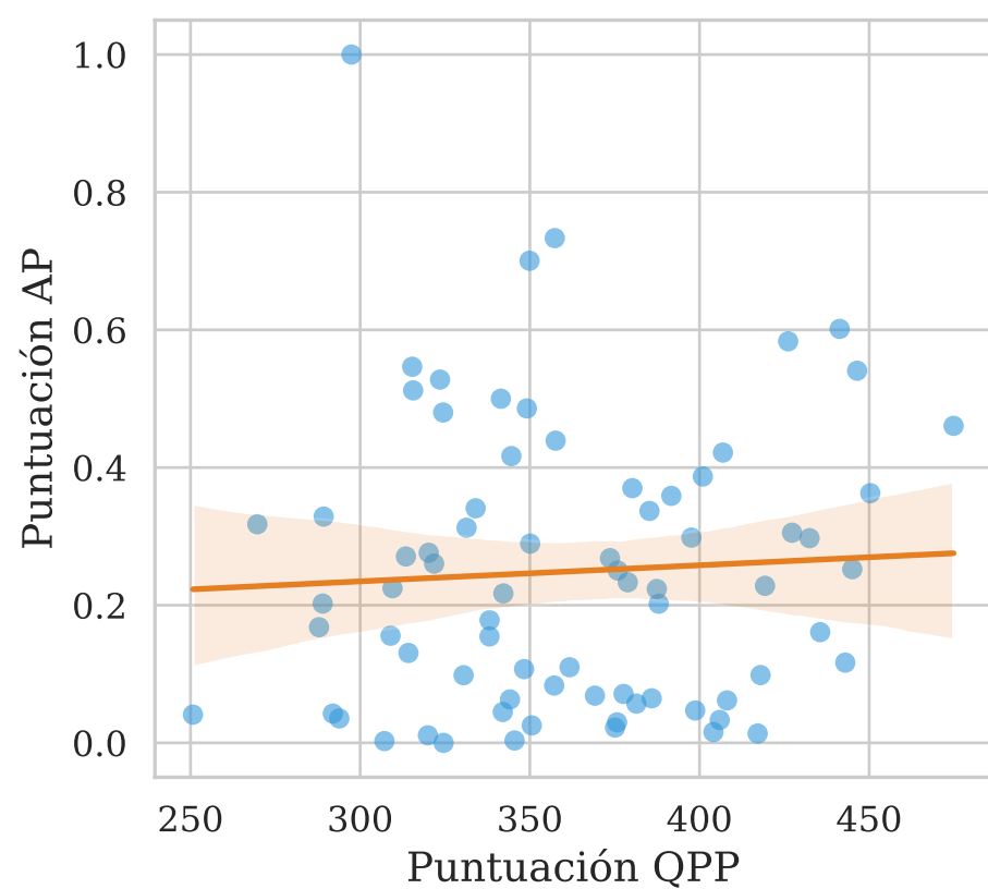
UEF-Clarity \tau = 0.1791
