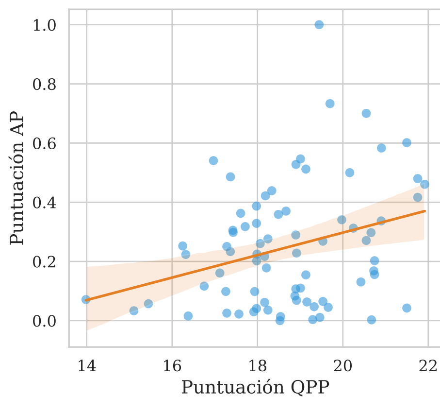
Clarity \tau = 0.0573
