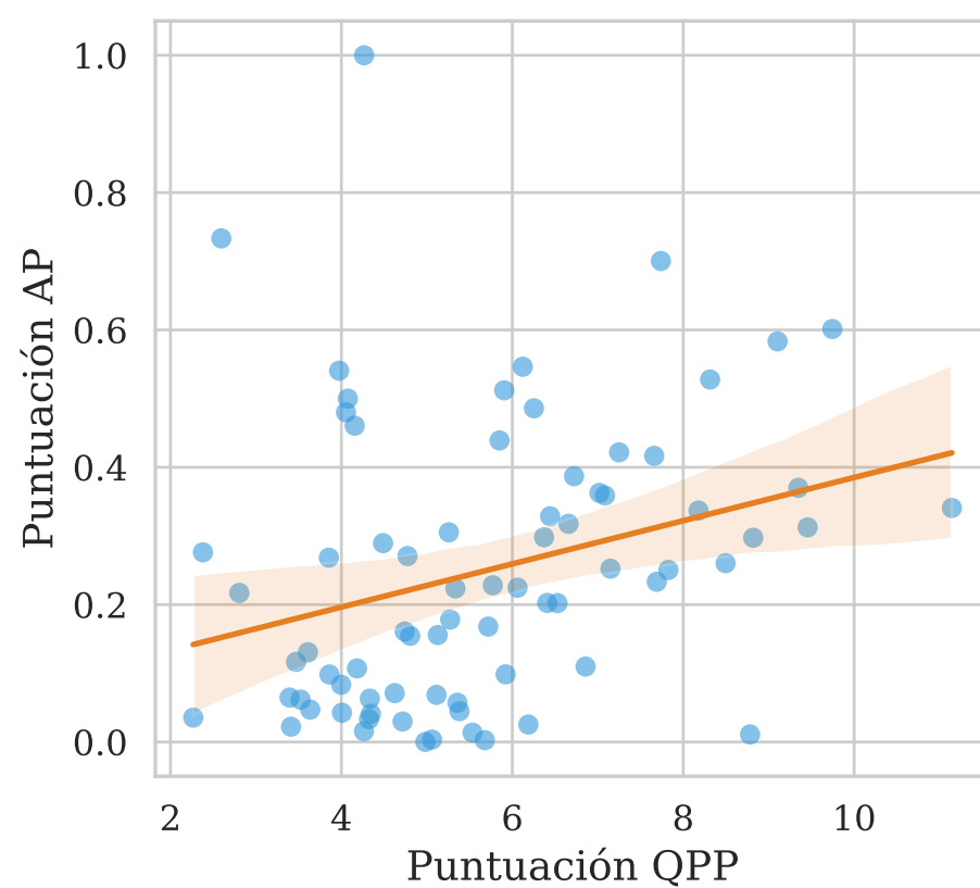
UEF-WIG \tau = 0.3816
