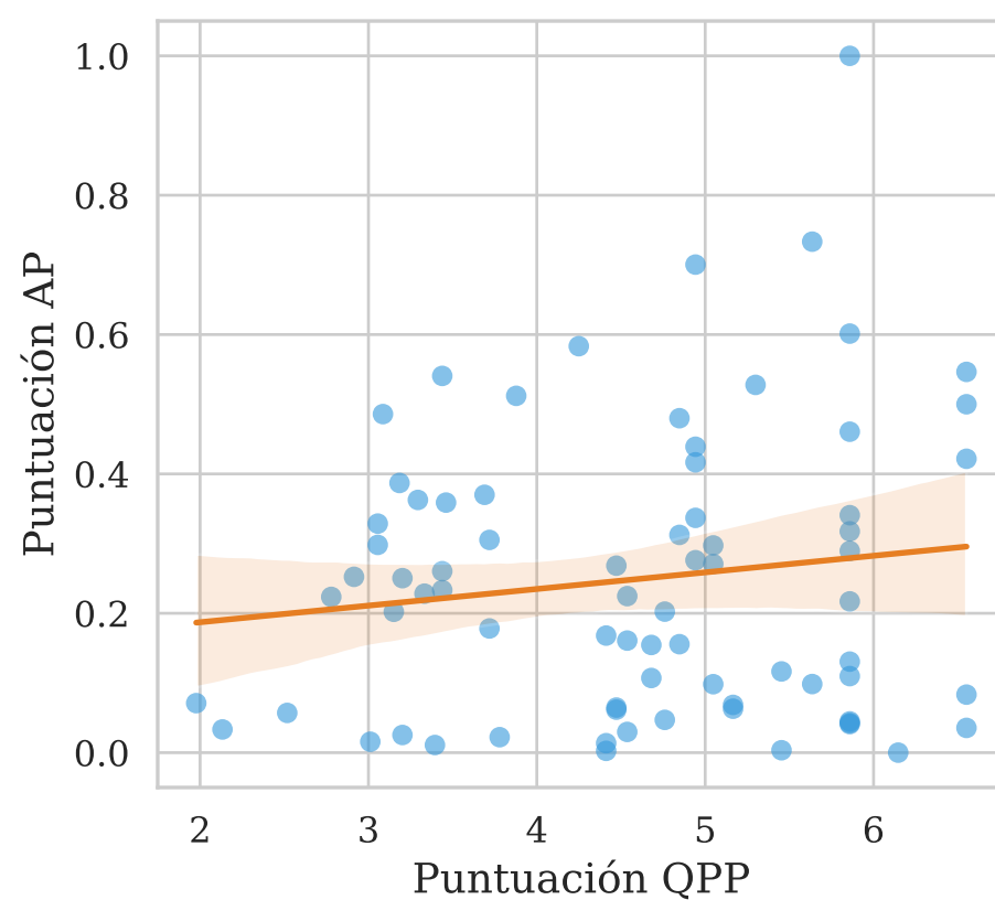
WIG \tau = 0.2605
