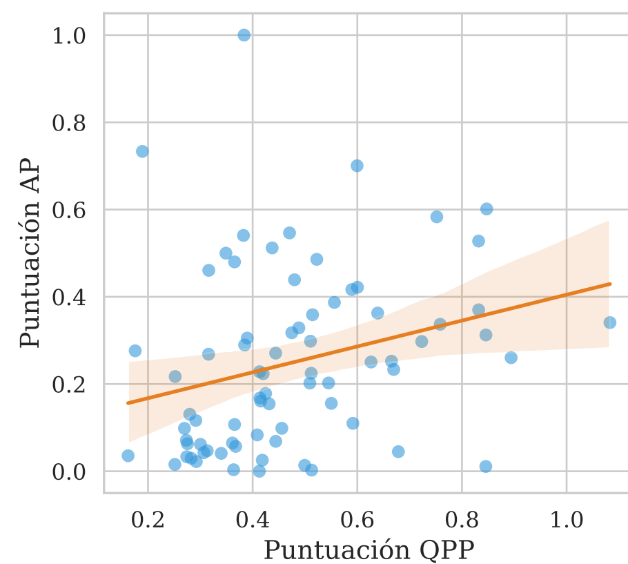
UEF-NQC \tau = 0.3715
