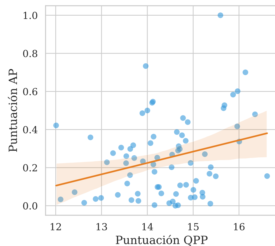
NQC \tau = 0.2656
