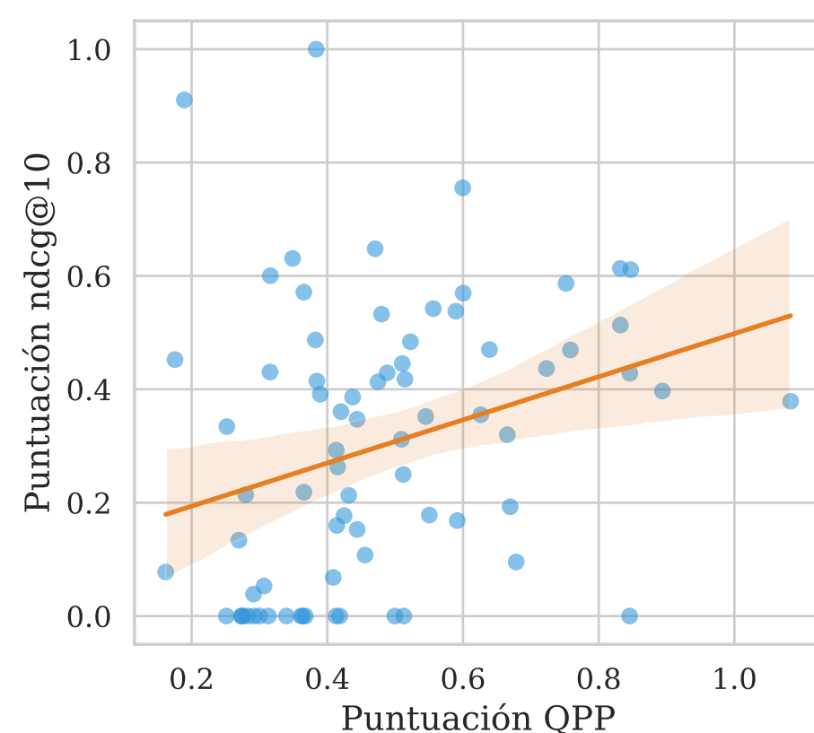
NQC \tau = 0.2709
