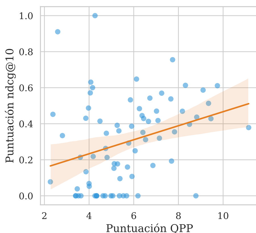
WIG \tau = 0.2627
