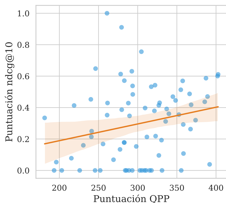
UEF-Clarity \tau = 0.1726
