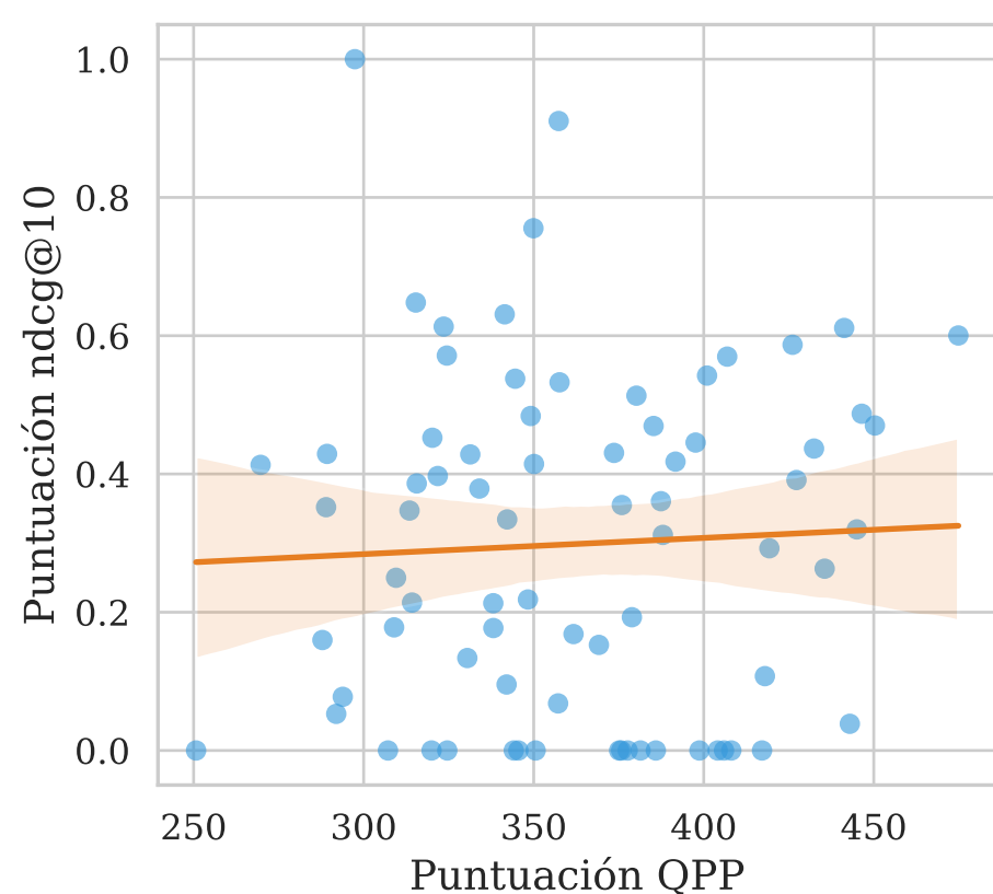
Clarity \tau = 0.0418
