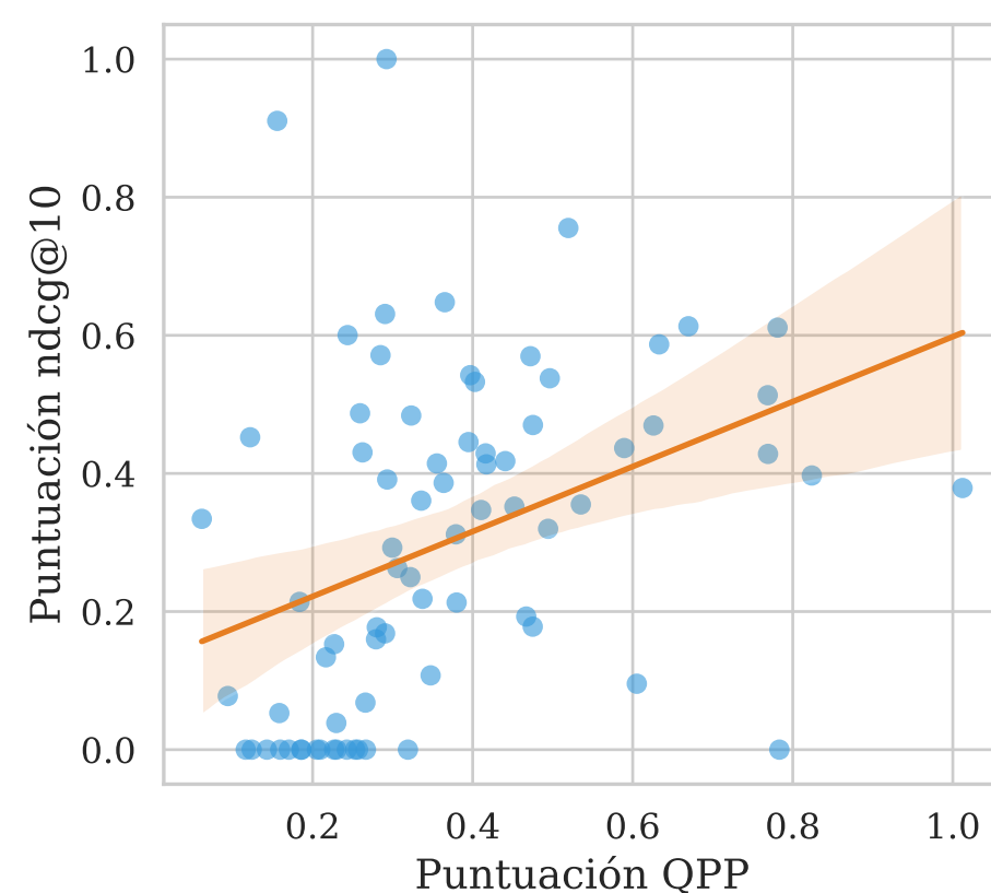
UEF-NQC \tau = 0.3655
