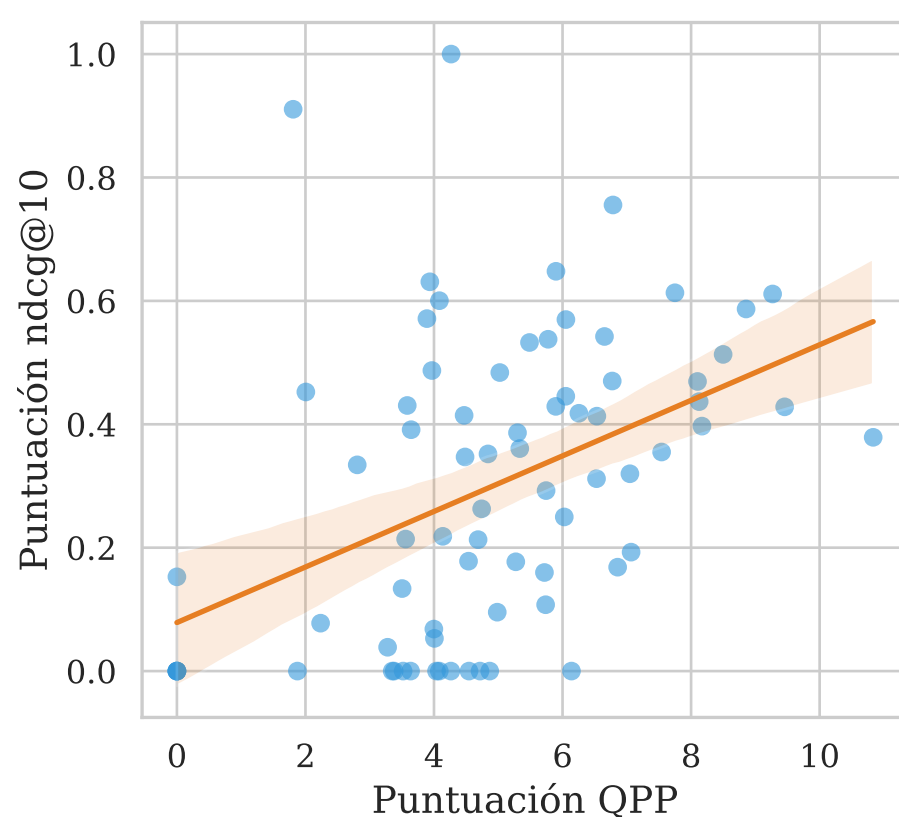
UEF-WIG \tau = 0.3453
