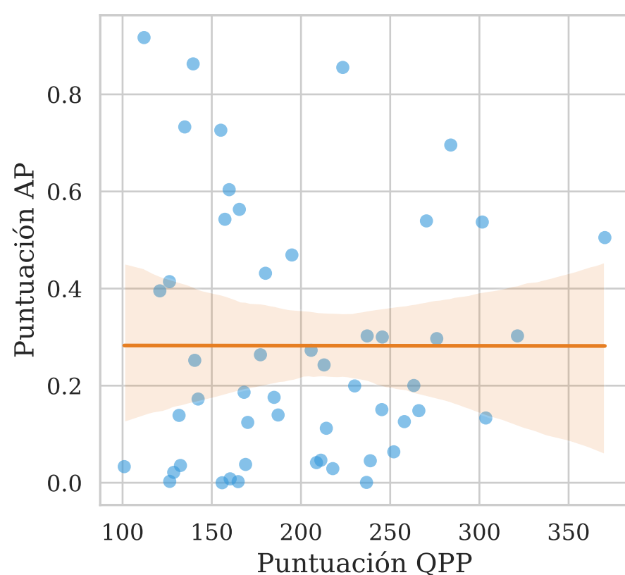
UEF-Clarity \tau = 0.0557
