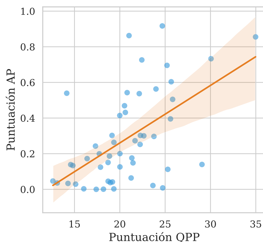
WIG \tau = 0.3851
