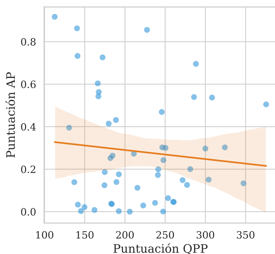
Clarity \tau = -0.0118
