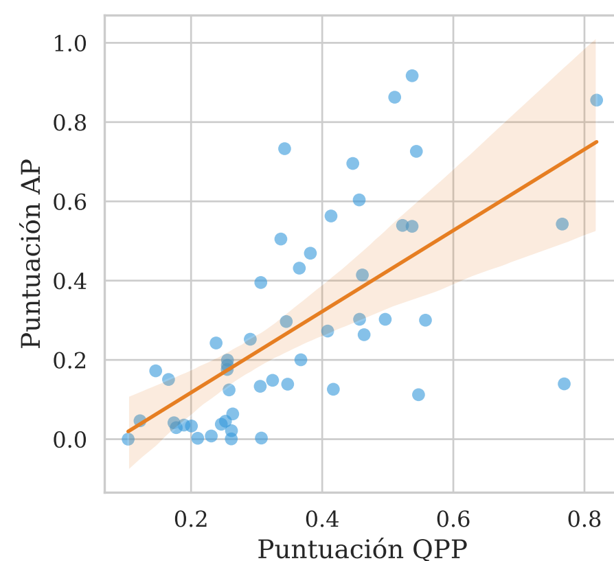
UEF-NQC \tau = 0.5075
