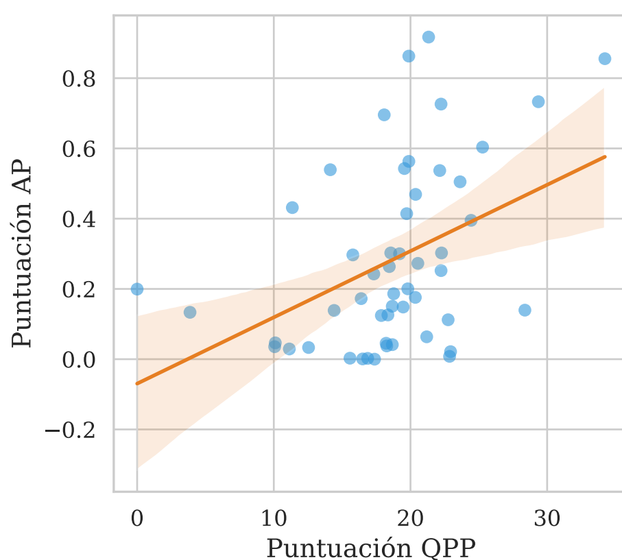
UEF-WIG \tau = 0.3035
