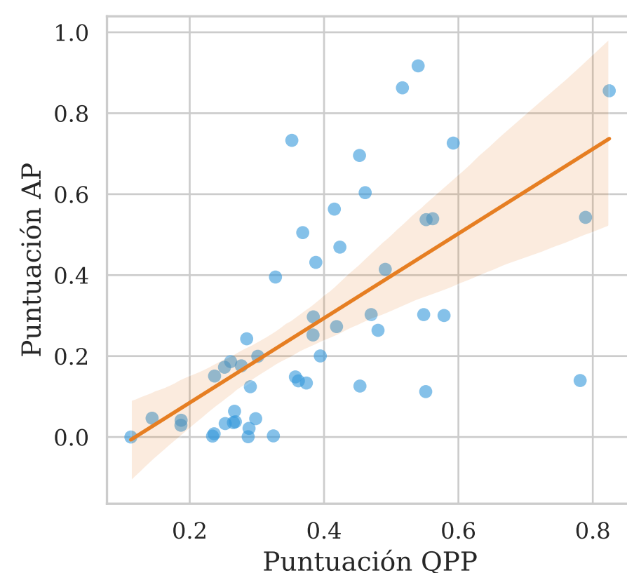
NQC \tau = 0.5357
