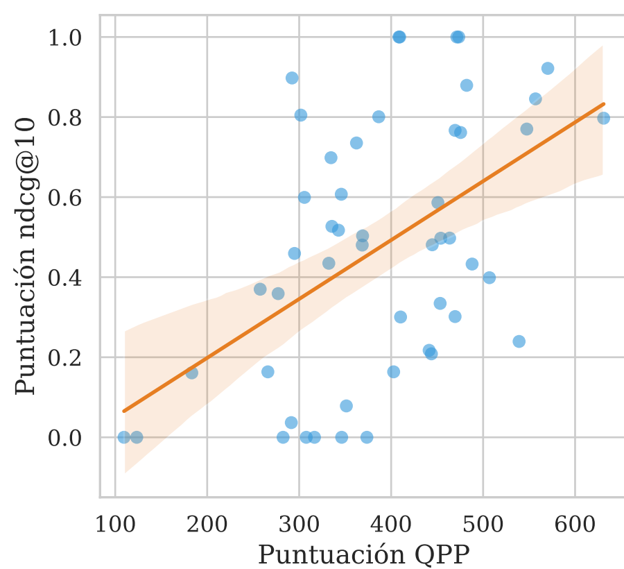
UEF-Clarity \tau = 0.3312
