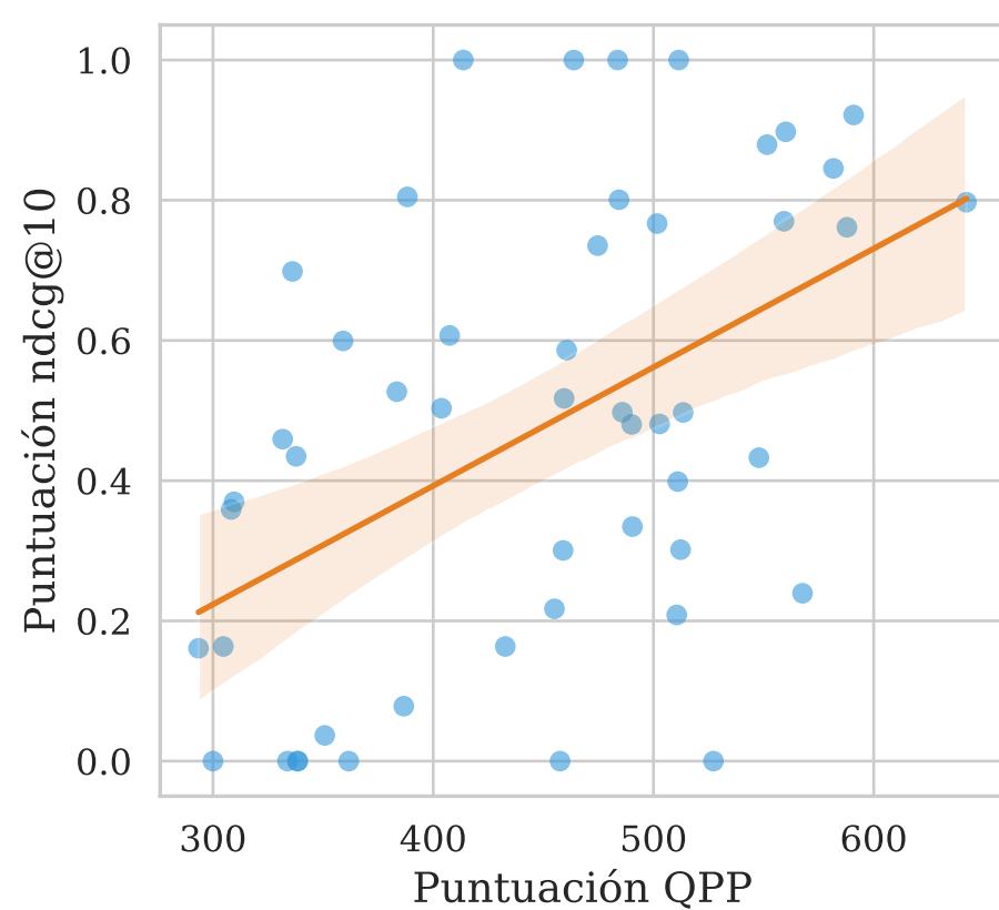
Clarity \tau = 0.3196
