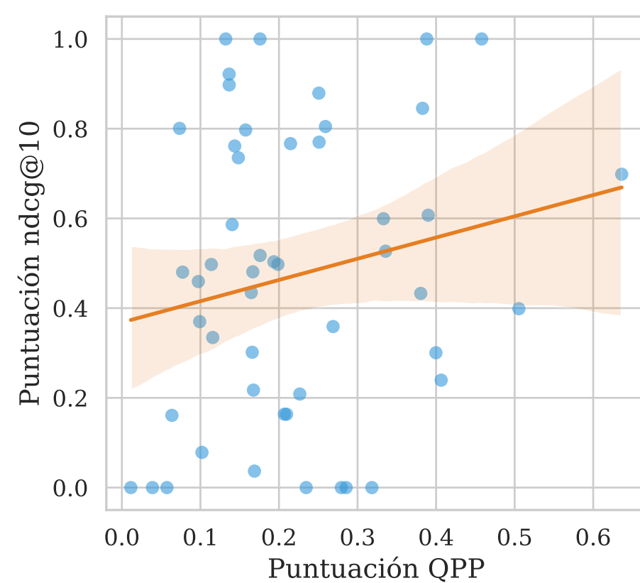
NQC \tau = 0.0933
