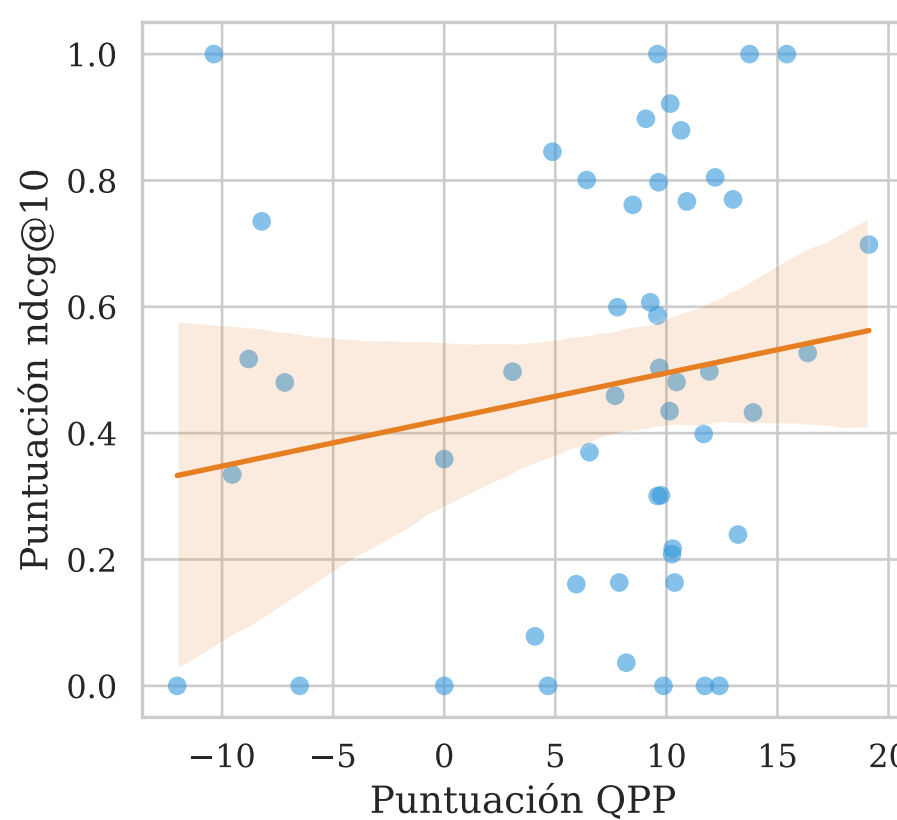
UEF-WIG \tau = 0.1338
