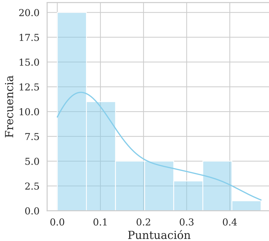
AP
