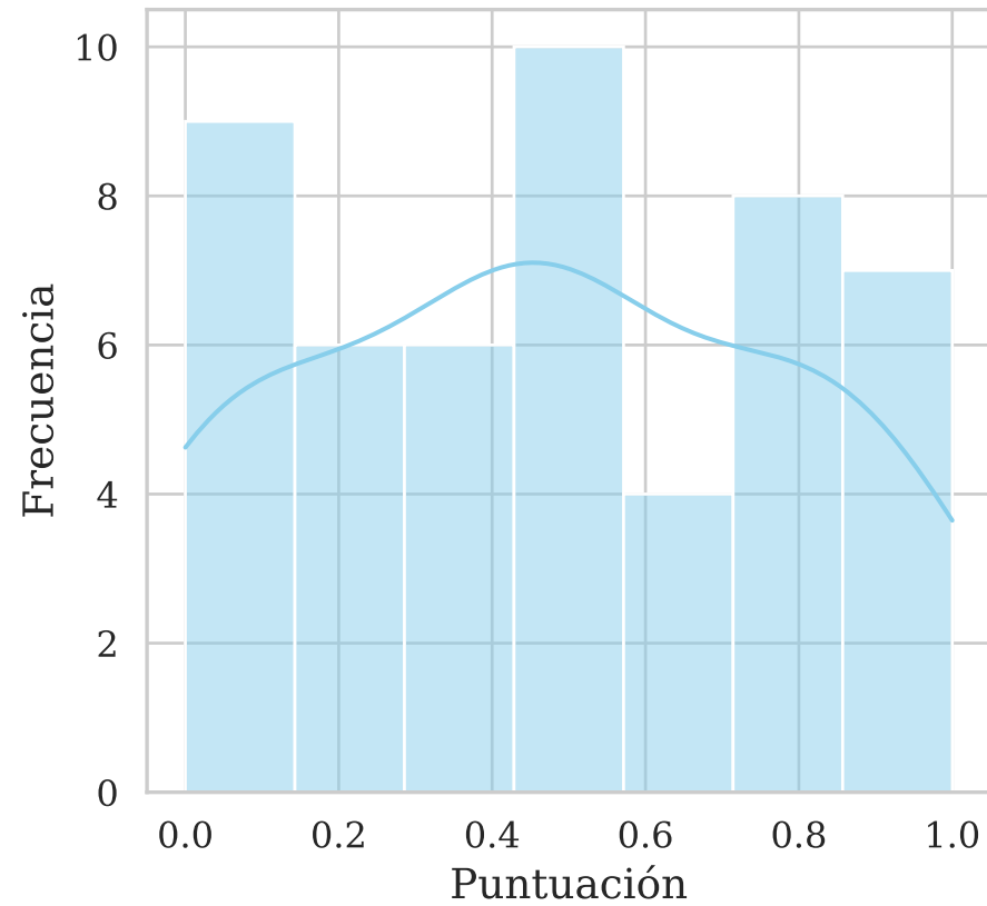
nDCG@10
