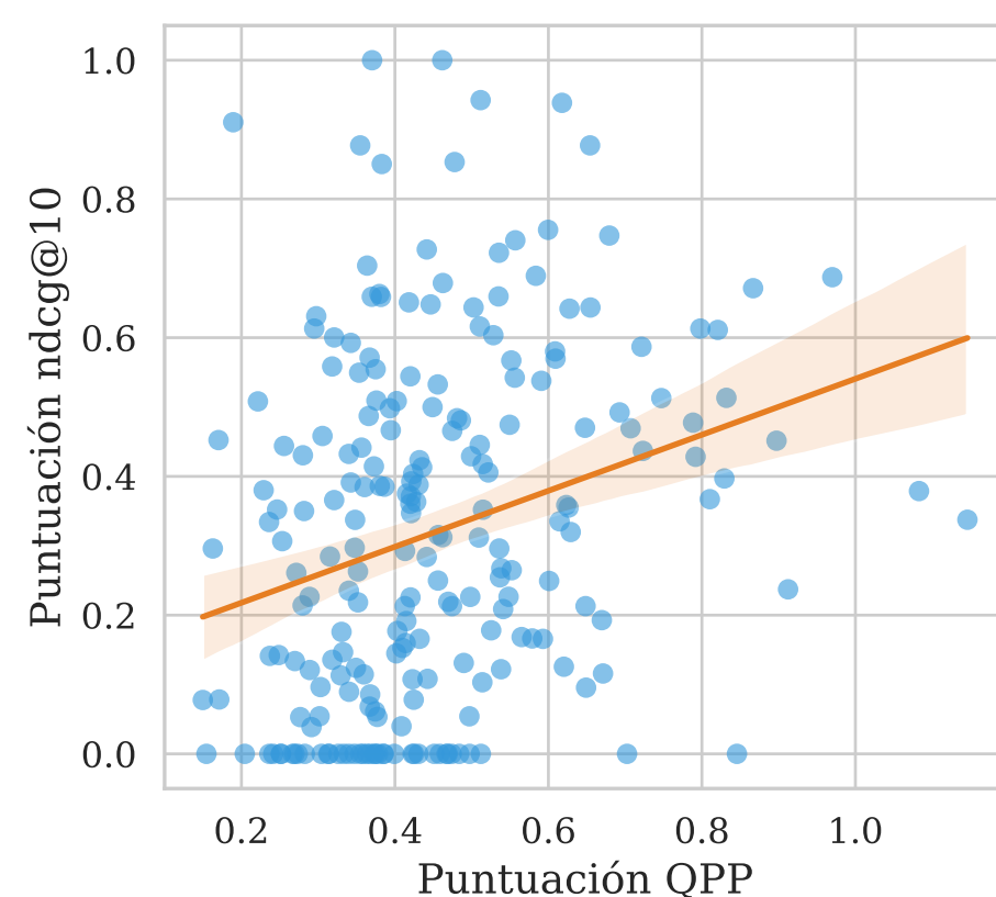
NQC \tau = 0.2103
