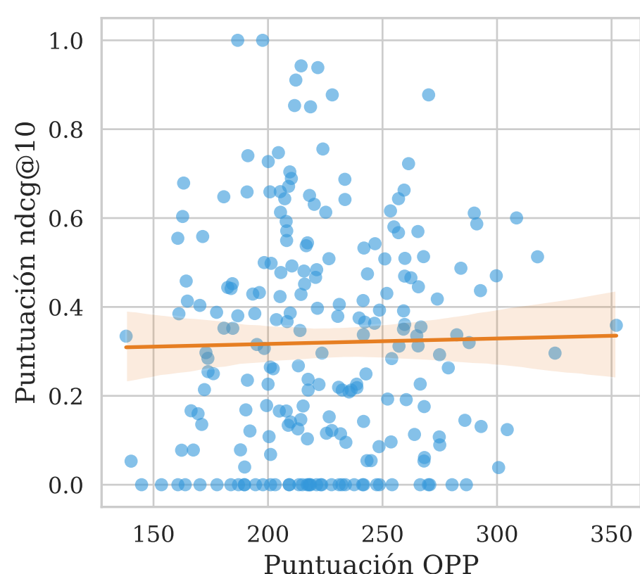
UEF-Clarity \tau = 0.0108
