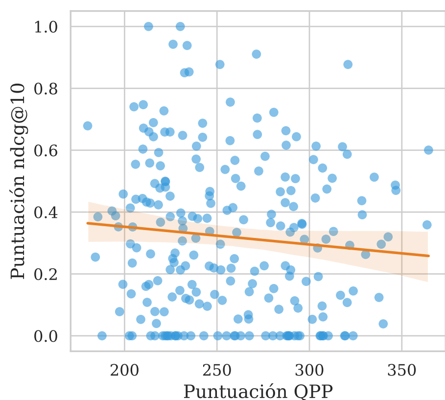
Clarity \tau = -0.0690
