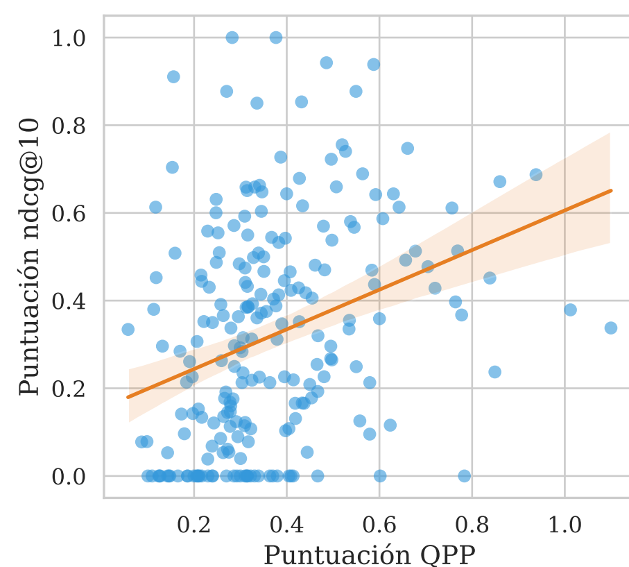
UEF-NQC \tau = 0.2583
