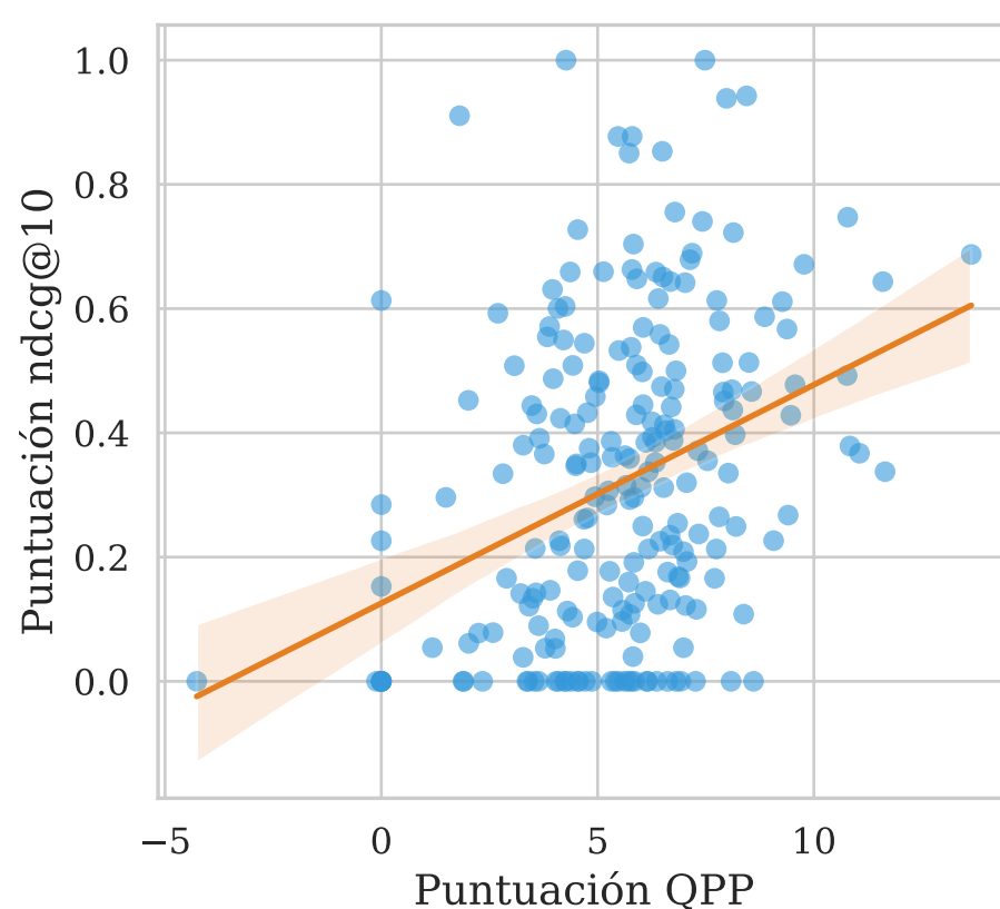
UEF-WIG \tau = 0.2328
