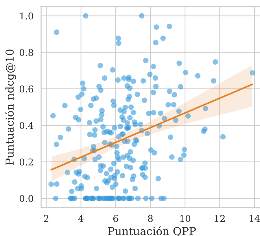
WIG \tau = 0.2224
