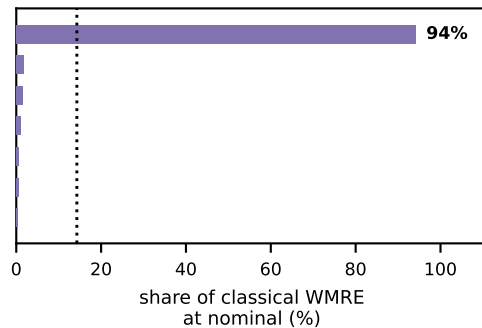
Methyl butanoate
