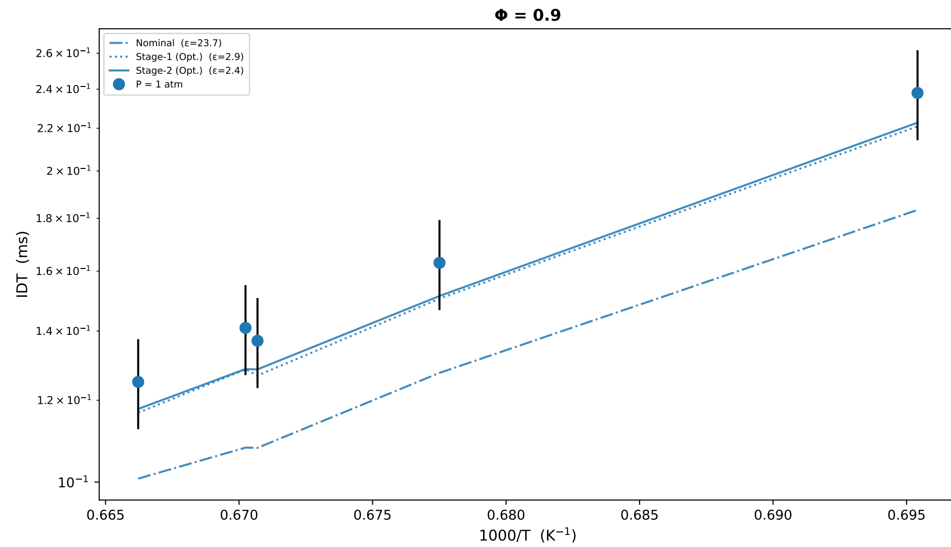
Ignition Delay Time — Mechanism Comparison
