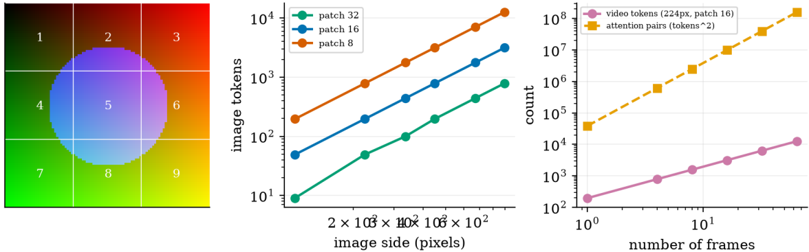
96x96 image, 32x32 patches: 9 tokens
