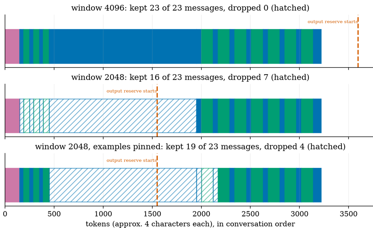
A conversation drawn to scale (purple = system prompt, blue = user messages, green = assistant messages; the long blue block is retrieved documents). Top: a 4096-token window holds everything (3220 tokens plus a 500-token reserve for the reply). Middle: with a 2048-token window the oldest messages are dropped first: all three few-shot examples and the retrieved documents disappear (hatched), exactly the parts the model needs. Bottom: pinning the three examples keeps them, but the retrieved documents (1500 tokens) still cannot fit.
