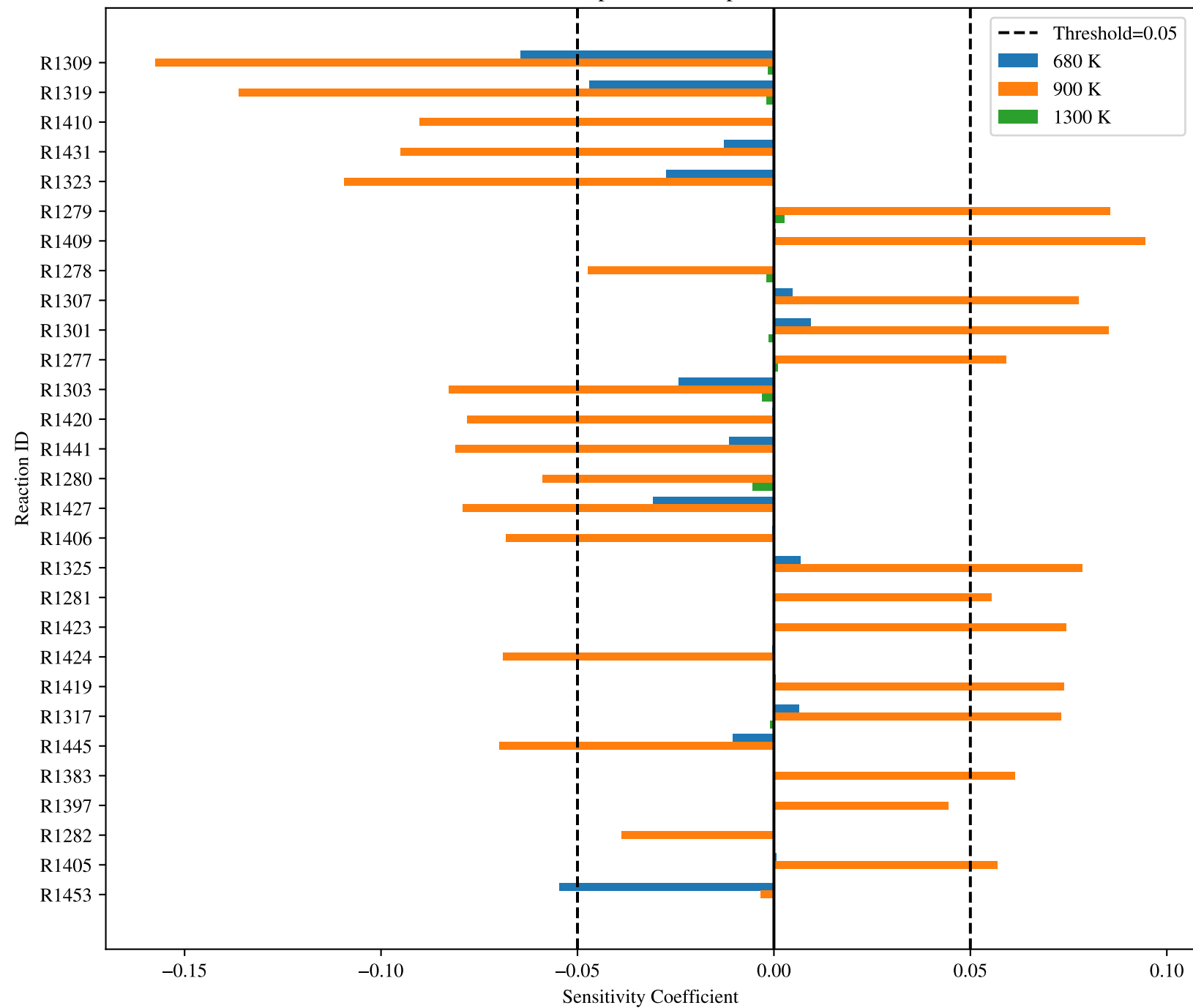
LTC Temperature Comparison
