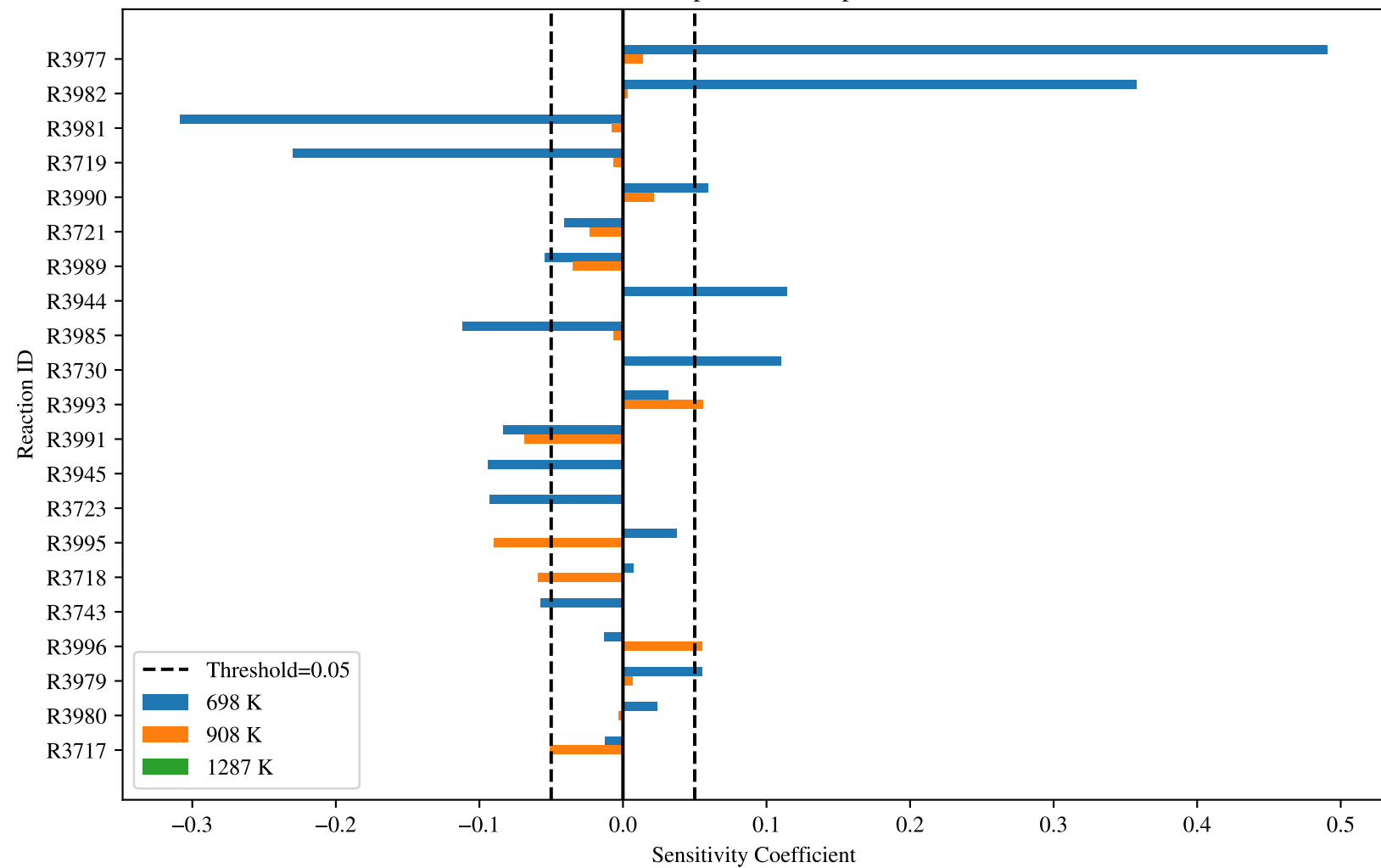
LTC Temperature Comparison
