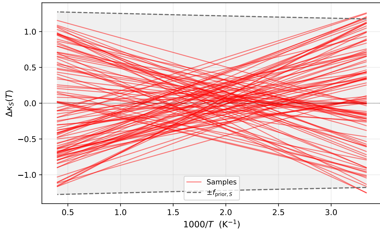
Perturbation curves \Delta\kappa_S(T)
