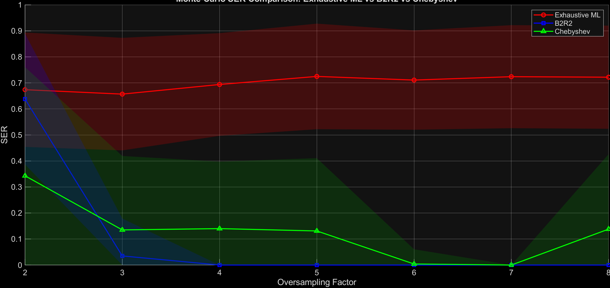
Monte-Carlo SER Comparison: Exhaustive ML vs B2R2 vs Chebyshev
