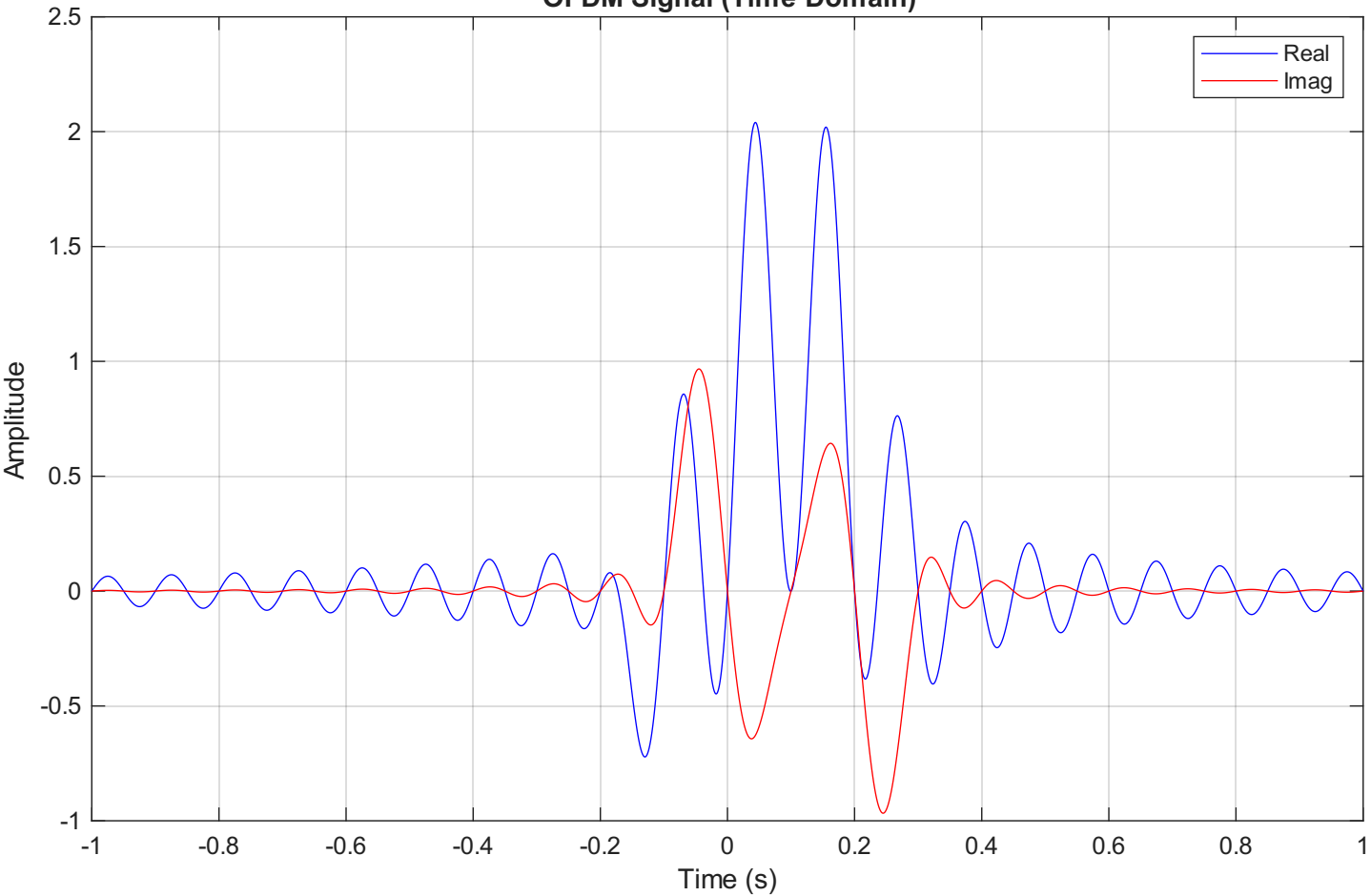
OFDM Signal (Time Domain)
