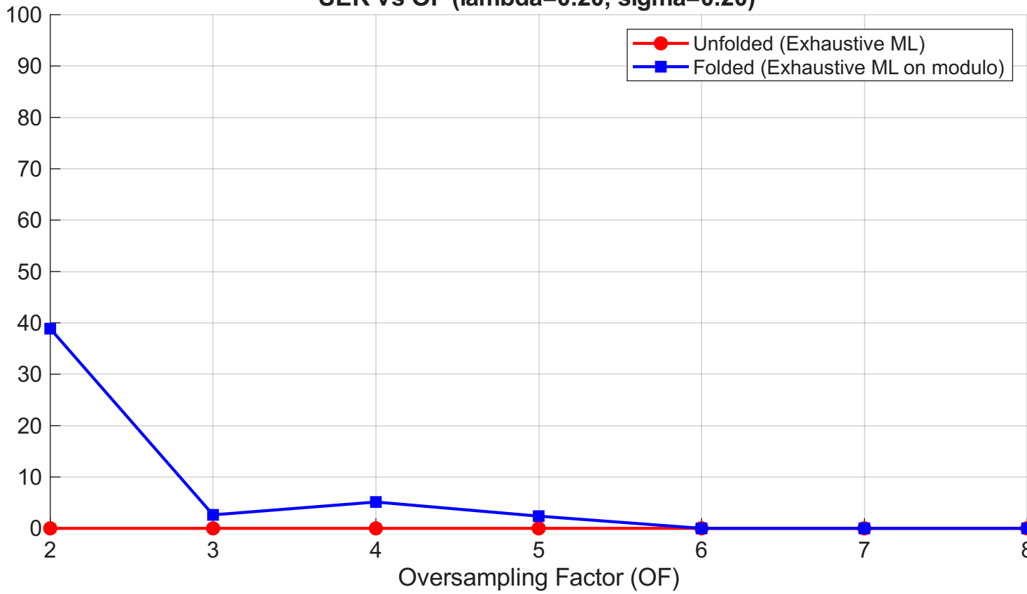
SER vs OF ( \lambda=0.20 , \sigma=0.20 )
