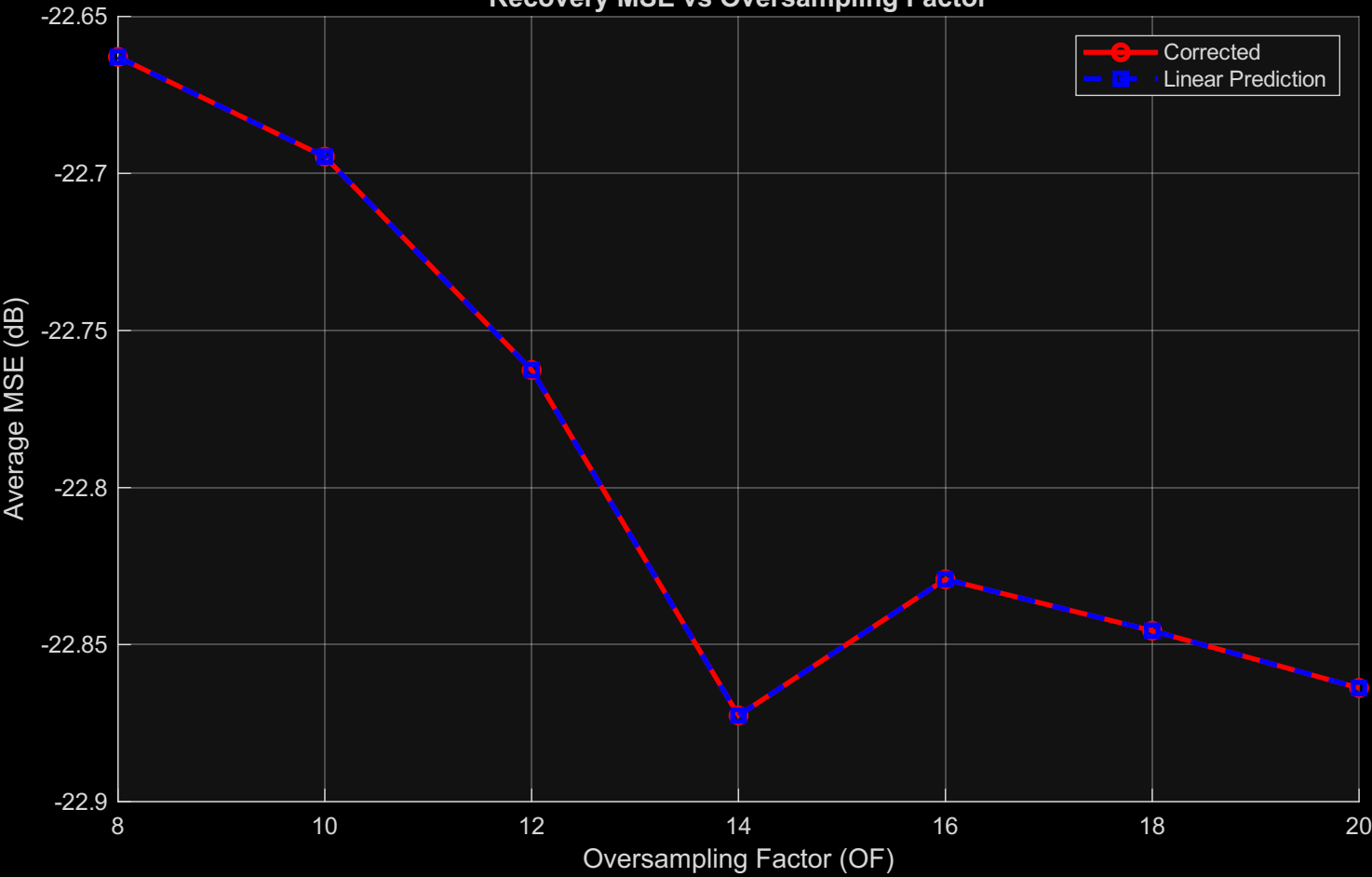
Recovery MSE vs Oversampling Factor
