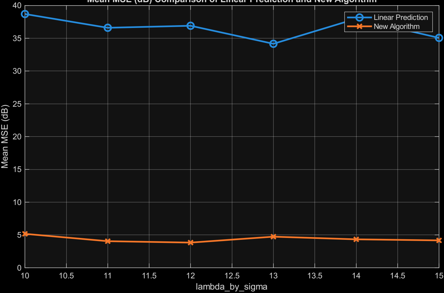
Mean MSE (dB) Comparison of Linear Prediction and New Algorithm
