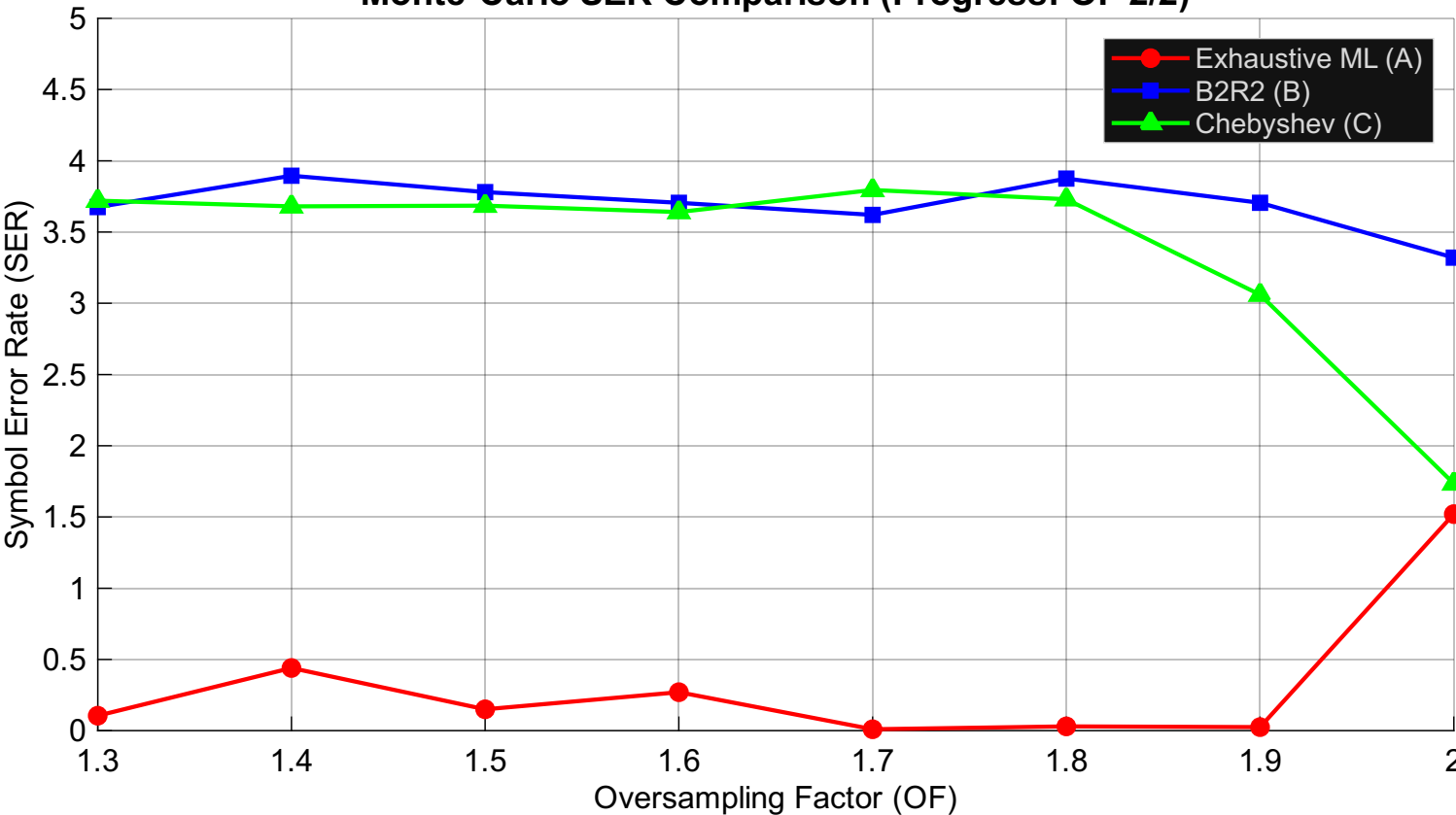
Monte-Carlo SER Comparison (Progress: OF 2/2)
