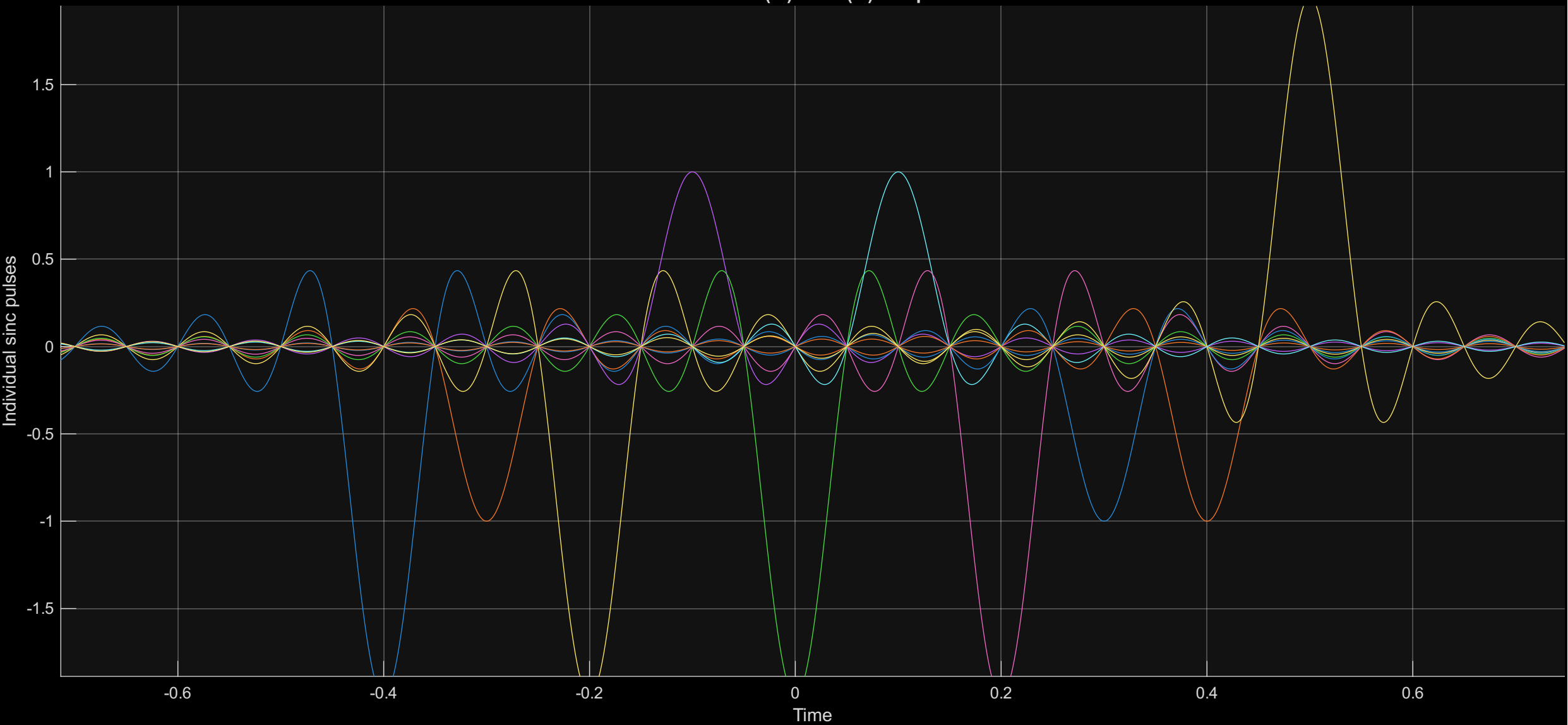
Individual CoS(m) * sinc(...) components
