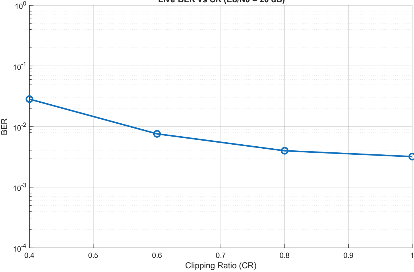
Live BER vs CR (Eb/N0 = 20 dB)
