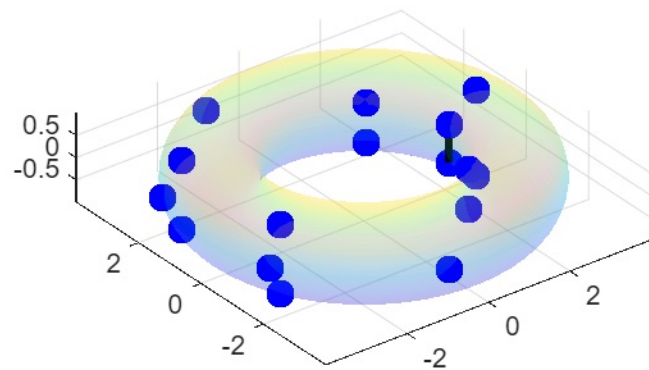
OFDM ( d_{\min}=0.0469 )
