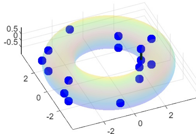
OFDM ( d_{\min}=0.0469 )
