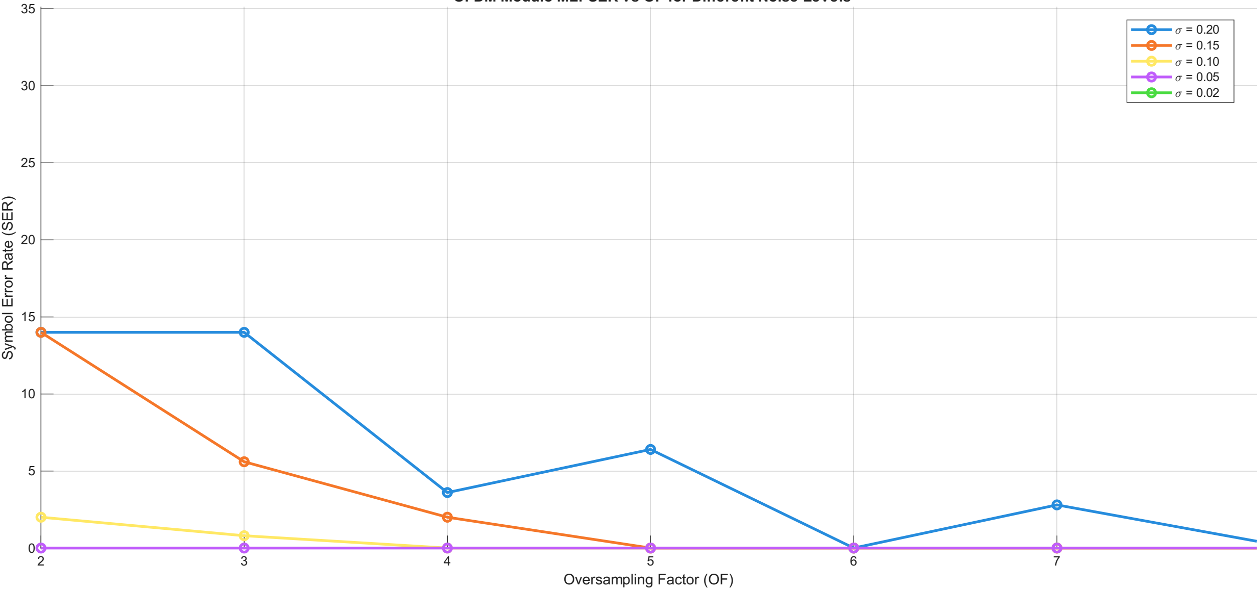
OFDM Modulo ML: SER vs OF for Different Noise Levels
