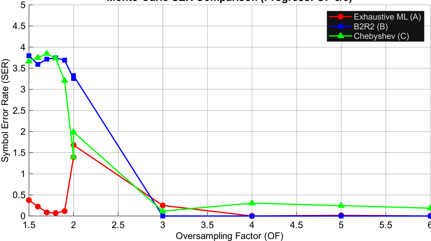
Monte-Carlo SER Comparison (Progress: OF 6/6)
