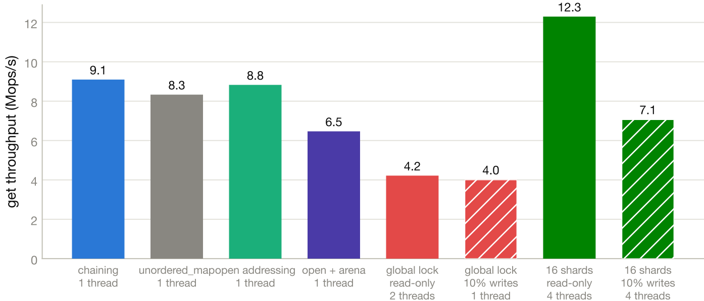
1M keys, 16B values — single-threaded stores vs concurrent wrappers at their best thread count
