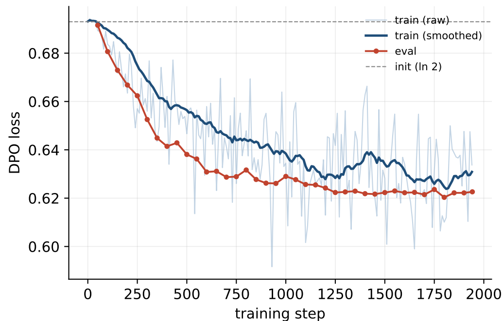
Loss
