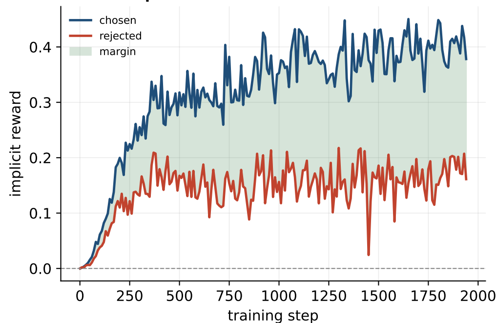
Reward separation
