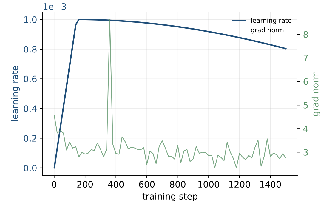
LR schedule + grad norm
