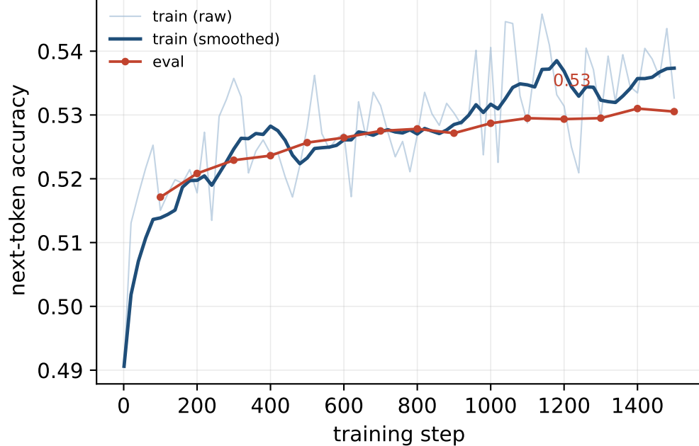
Token accuracy
