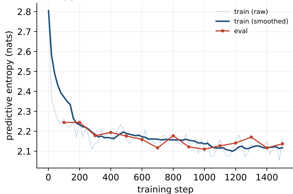
Entropy
