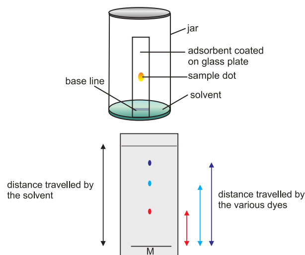
Fig. 3.8 (b) Developed chromatogram.
