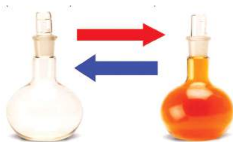
Figure 12.3 : \text{N}_2\text{O}_4 conversion to \text{NO}_2
