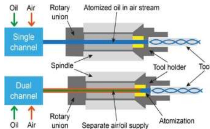
Figure: MQL internal delivery system[23]
