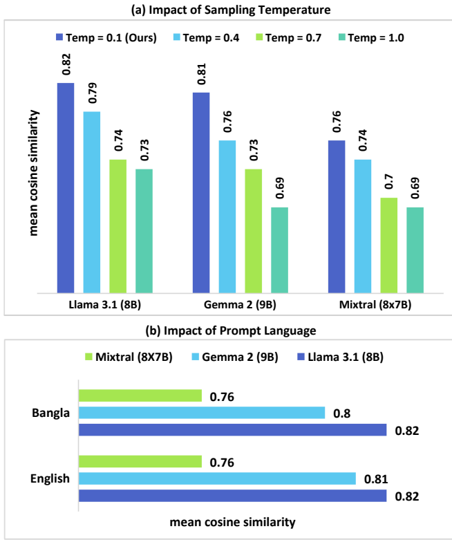
Fig. 5: The impact of (a) sampling temperature and (b) prompt language on the responses generated by the Advanced RAG.
